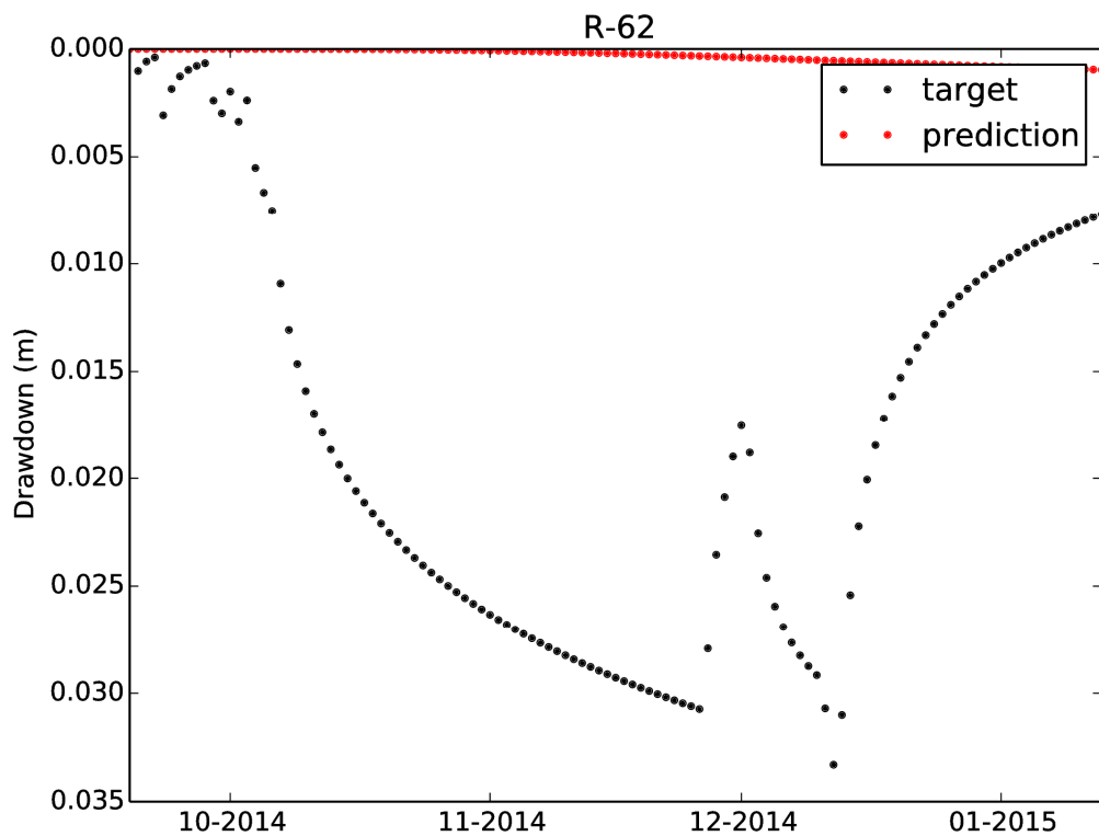
Figure A-6.0-17 Model calibration targets (black dots) and predictions (red dots) for the drawdown at R-62 to pumping at CrEX-1
