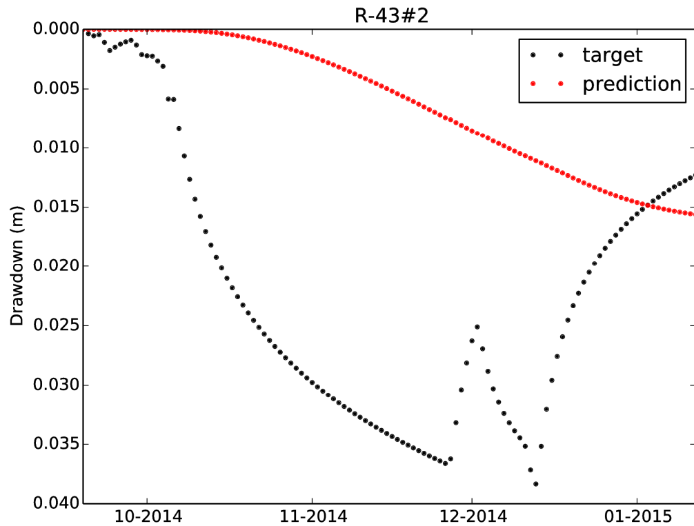
Figure A-6.0-10 Model calibration targets (black dots) and predictions (red dots) for the drawdown at R-43 screen 2 to pumping at CrEX-1
