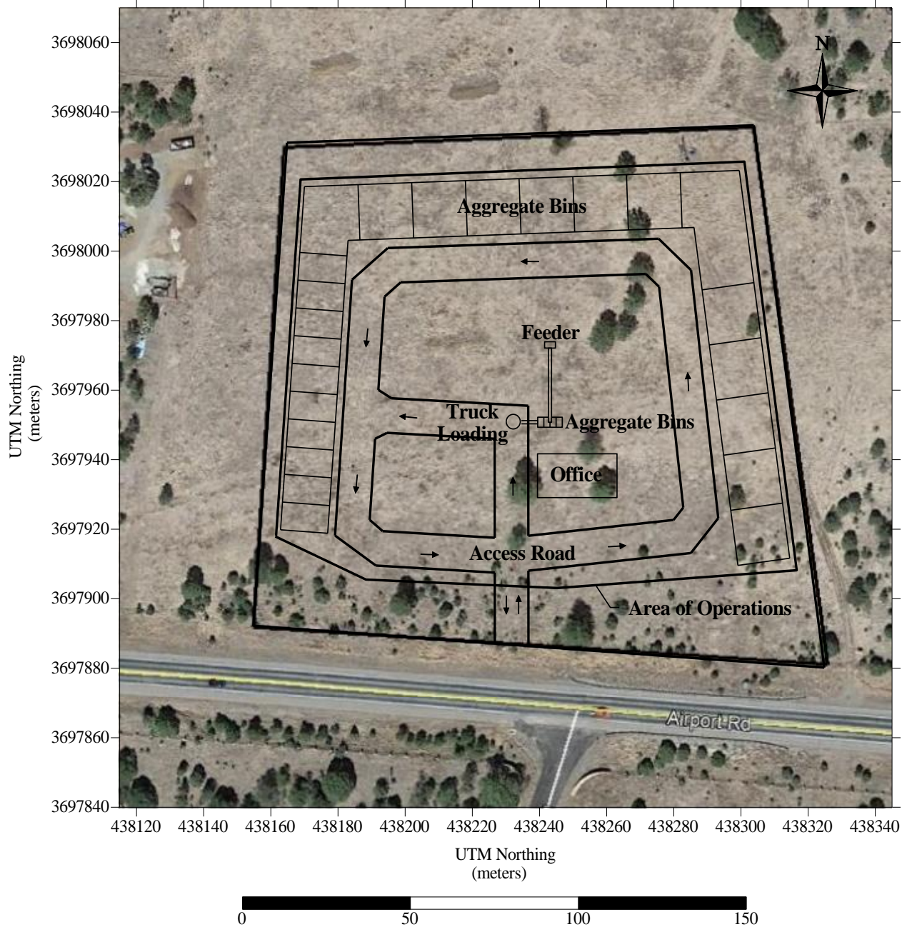
Figure 5-1: Alto CBP Site Plot Plan
