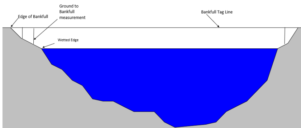
Figure 5. Bankfull and ground to bankfull tag line measurement
