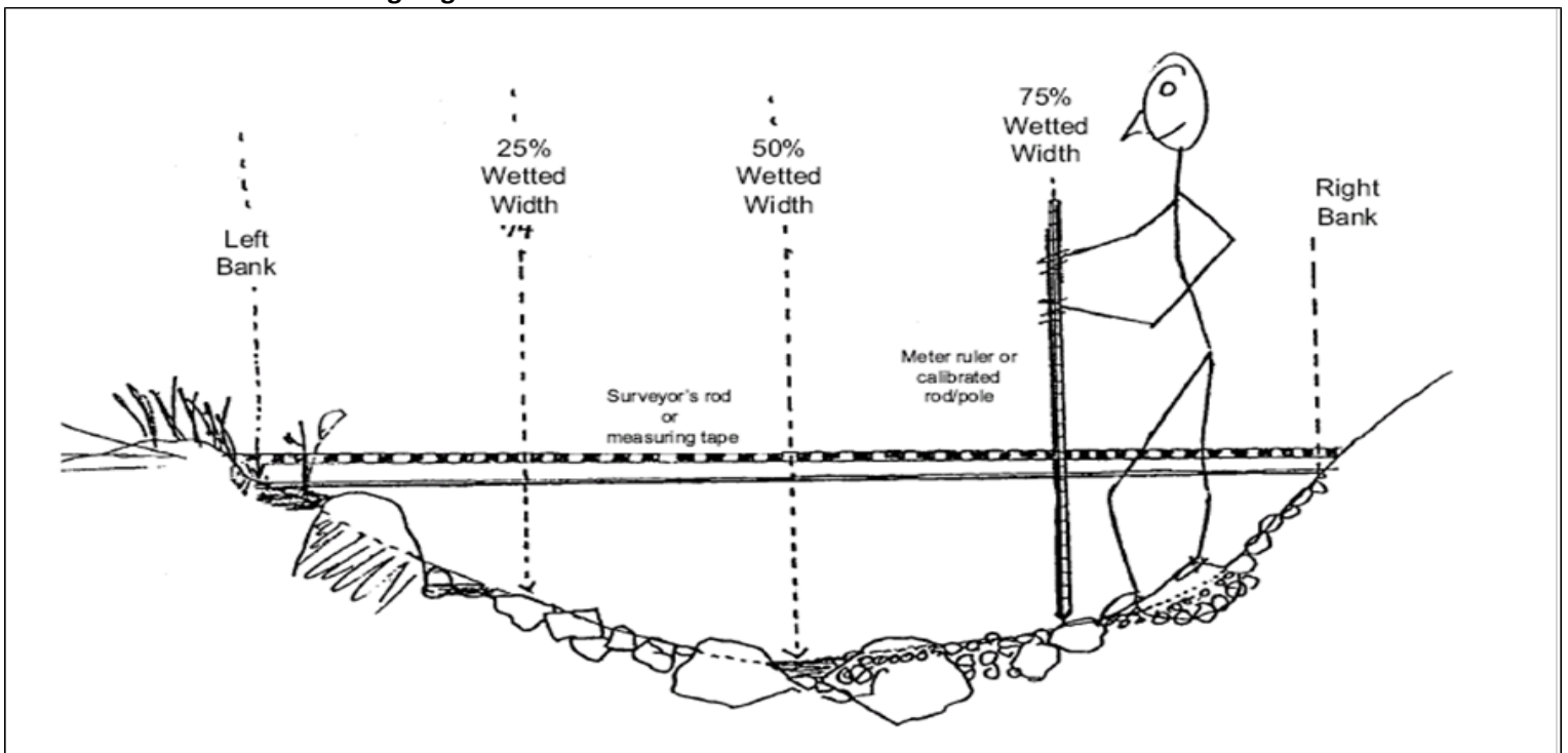
Figure 2. Substrate Sampling Cross-Section
