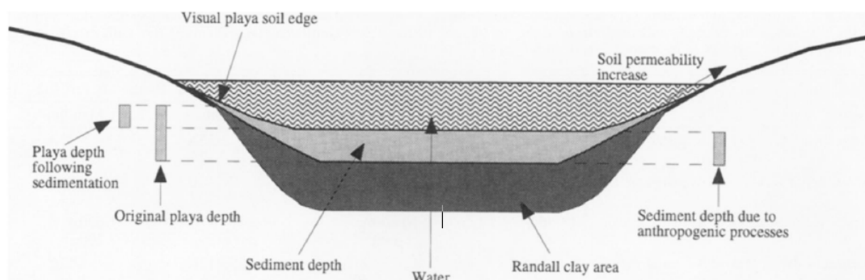
Figure 24. The Playa Soil Condition Index is measured from three soil pits augured or dug to 50 cm in depth in the playa bottom. The thickness of the sediment layer above the clay pan is determined by texture and color (from Luo et al. 1997).
