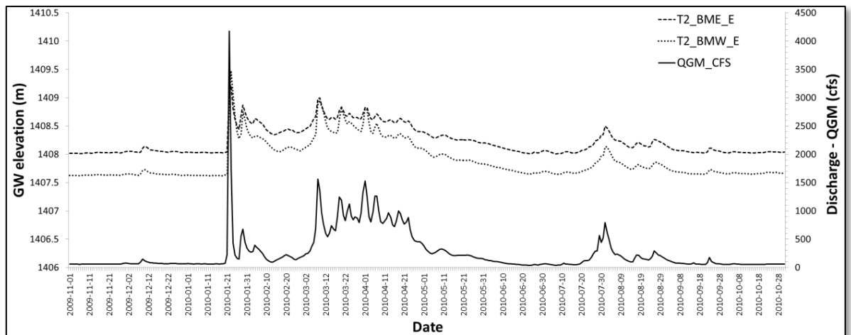
Figure 7. An example of stream flow and groundwater dynamics in water year 2010 on the Gila River near Gila, NM. Surface water flow includes discharge from the Gila River and Mogollon Creek (QGM) combined and groundwater (GW) elevations from two piezometer wells at the site (T2_BMW_E is closer to the channel and T2_BME_E is further). Modified from Muldavin and Varani (2018).
