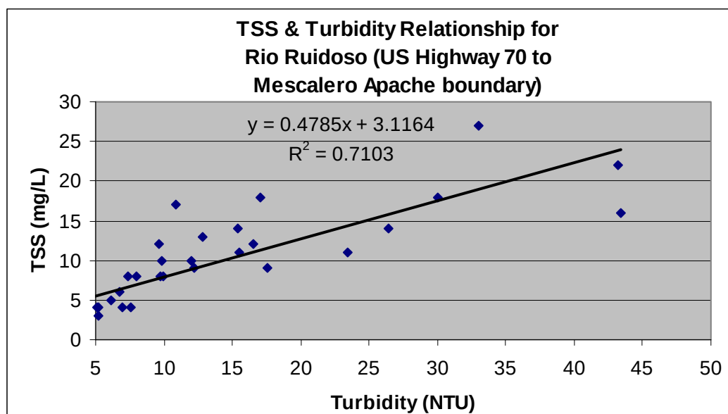
Figure 7.1 Relationship between TSS and Turbidity at Rio Ruidoso (US Highway 70 to Mescalero Apache boundary).
