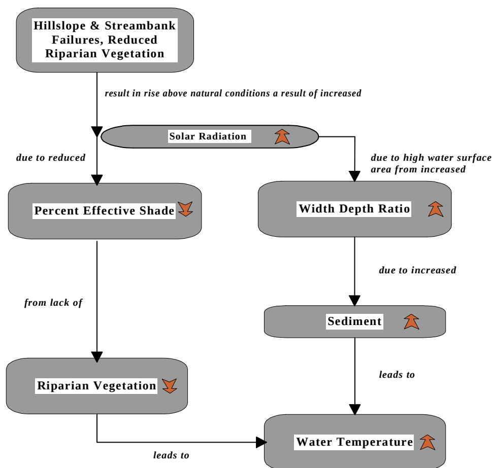
Figure 6.6 Factors That Impact Water Temperature
