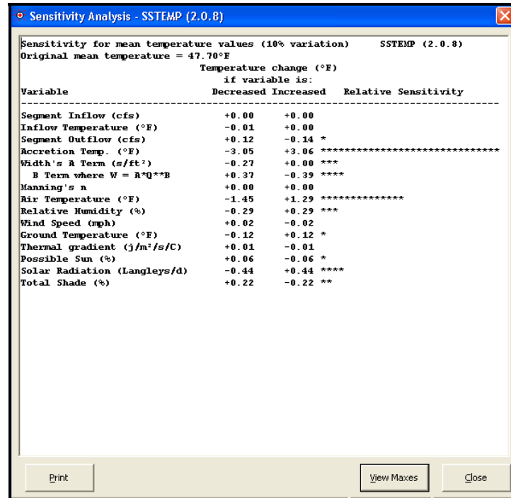
Figure 4.2 Example of SSTEMP sensitivity analysis for Gold Creek
