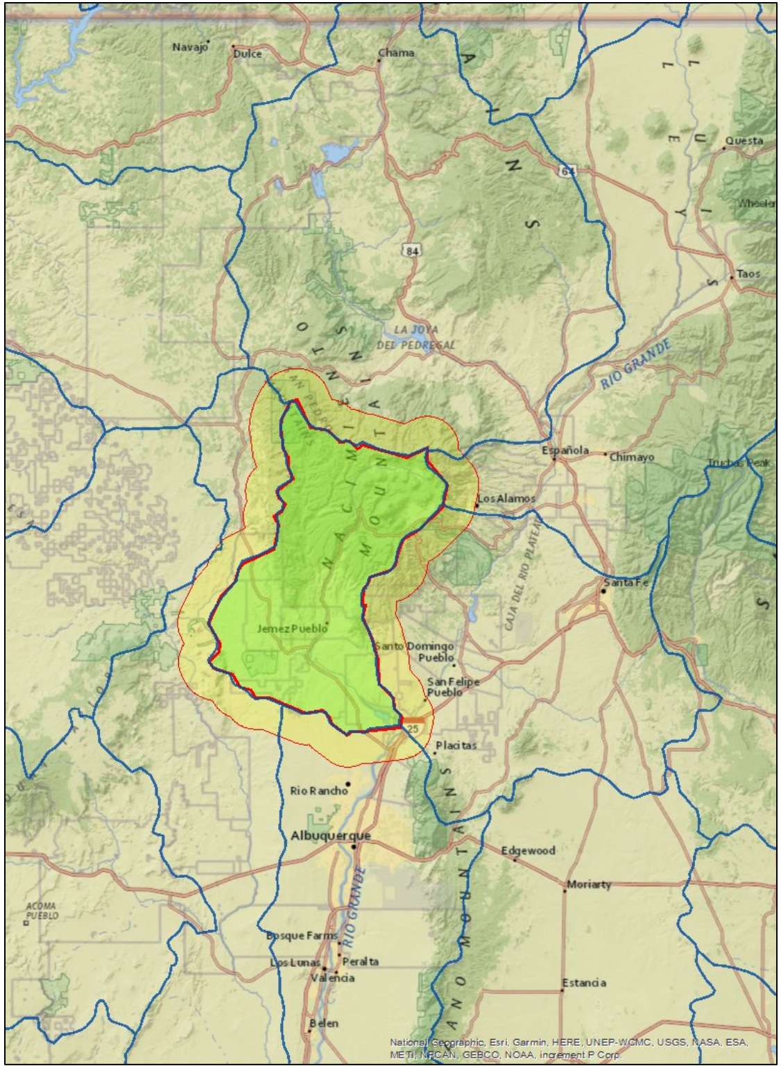
Figure 1: EJSreen map- US Geological Survey Jemez Hydrologic Unit Code 13020202
