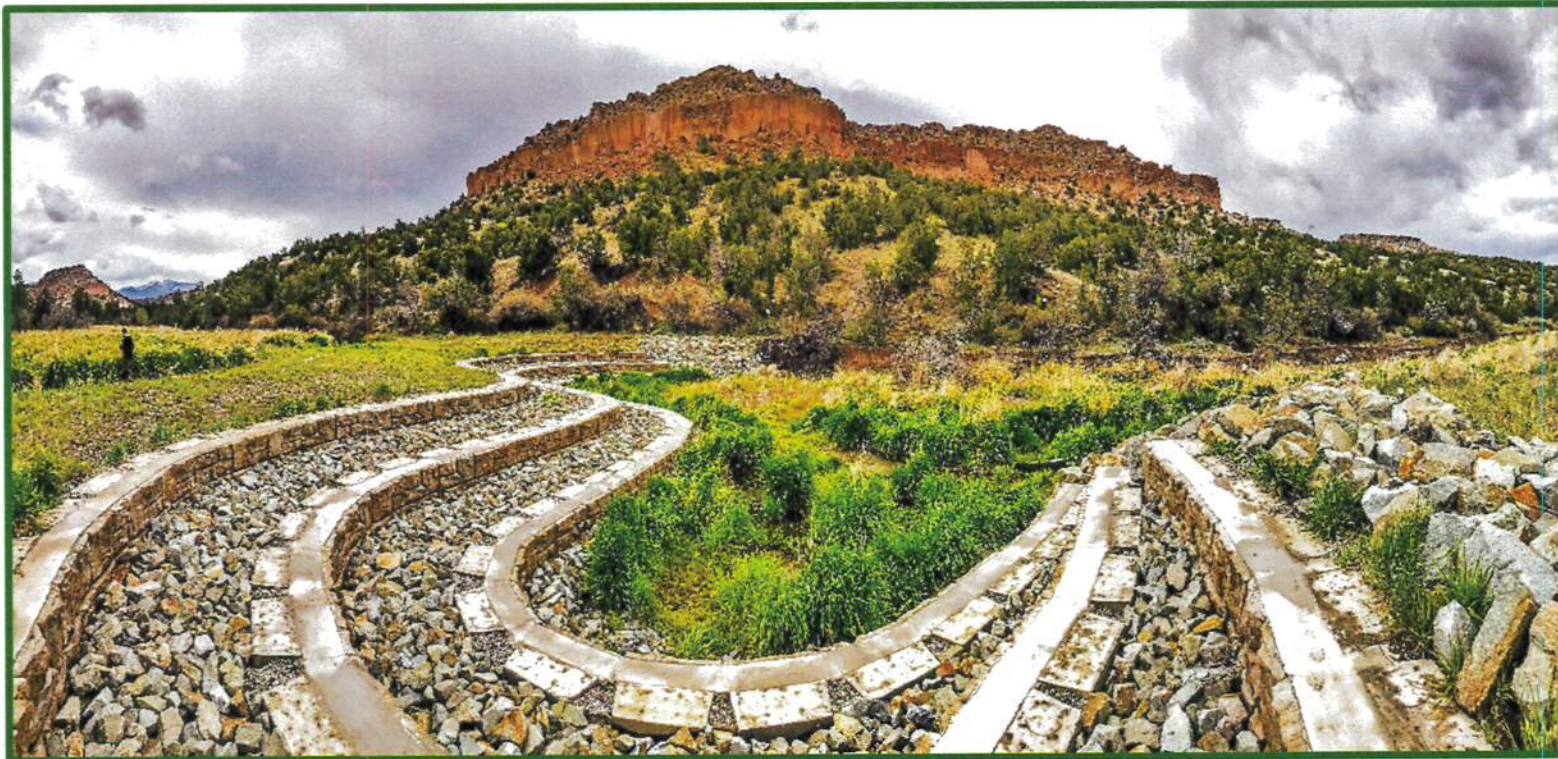
Redi-Rock wetland stabilization structure in Pueblo Canyon
