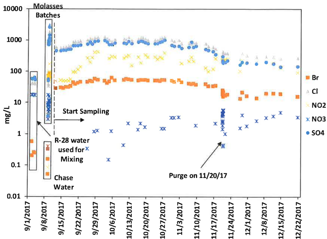
Figure 10 Concentrations of anions in R-28 molasses test as a function of time
