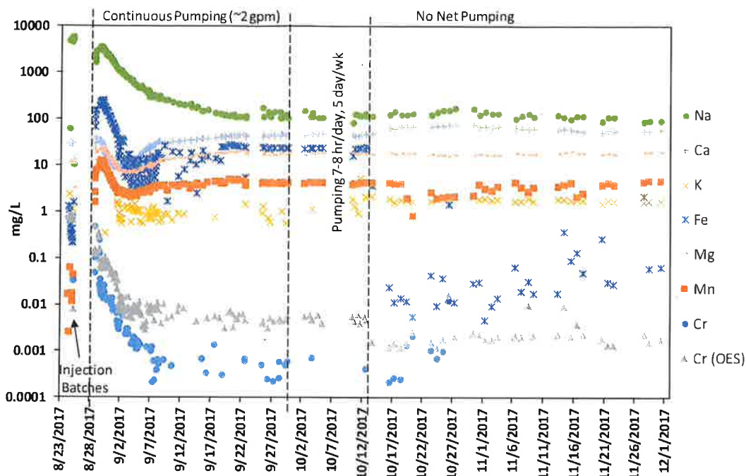
Figure 2 Concentrations of selected cations and metals in R-42 dithionite test as a function of time. The more reliable analytical results for chromium (inductively coupled plasma mass spectrometry [ICP-MS]) are lagging, so chromium results from ICP optical emission spectrometry (ICP-OES) are also shown.
