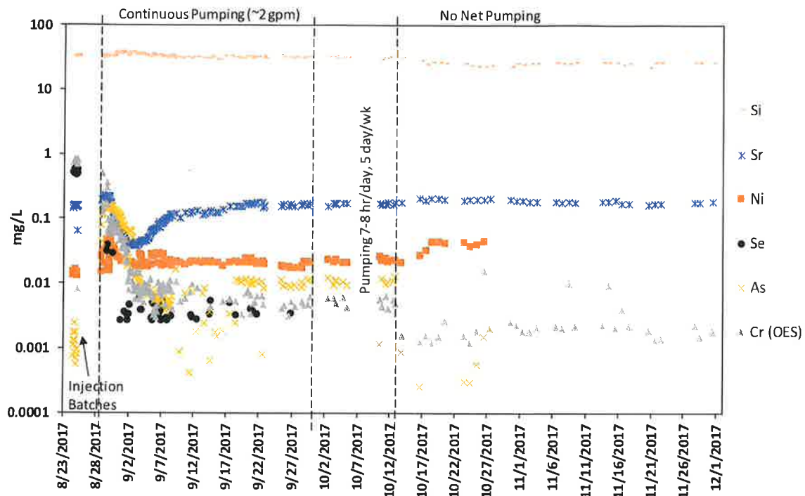
Figure 4 Concentrations of selected constituents during R-42 dithionite test as a function of time
