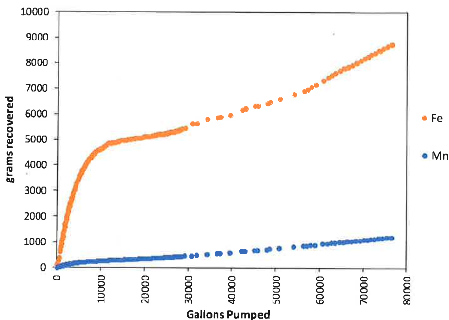
Figure 8 Recoveries of iron and manganese in R-42 dithionite test as a function of volume pumped
