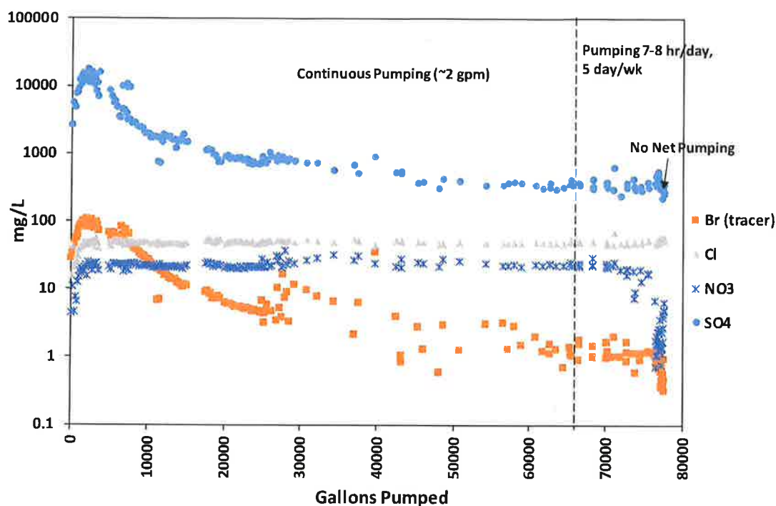
Figure 6 Data of Figure 5 plotted as a function of gallons pumped from R-42. Zero gallons pumped corresponds to 8/28/17 in Figure 5, and earlier data points from Figure 5 are not shown because these corresponded to injection batches that were not pumped from the well.
