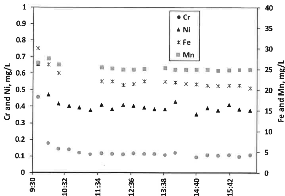
Figure 12 Concentrations of selected metals during the R-28 purge on 11/20/17
