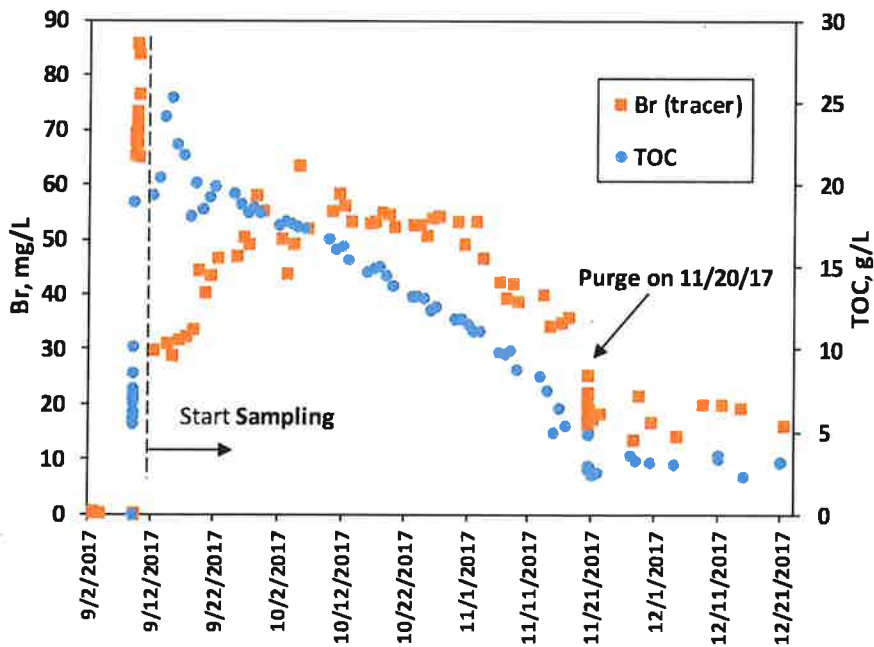
Figure 11 Concentrations of bromide and TOC in R-28 molasses test. Note that unlike other plots, concentration scales are not logarithmic.
