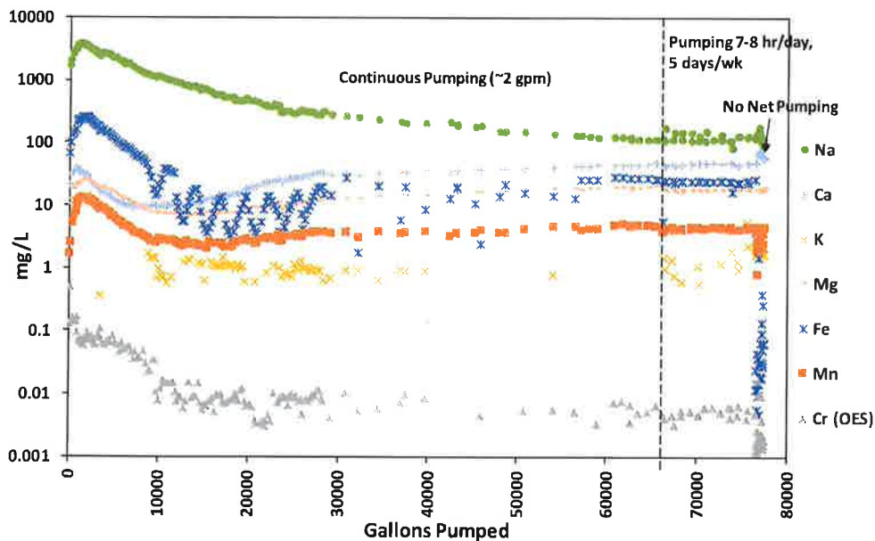
Figure 3 Data of Figure 2 plotted as a function of gallons pumped from R-42. Chromium data from ICP-MS (blue dots in Figure 2) are omitted. Zero gallons pumped corresponds to 8/28/17 in Figure 2, and earlier data points from Figure 2 are not shown because these corresponded to injection batches that were not pumped from the well.
