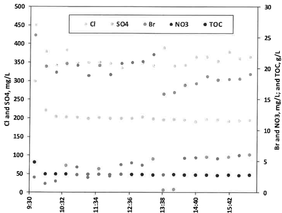
Figure 13 Concentrations of anions and TOC during R-28 purge on 11/20/17
