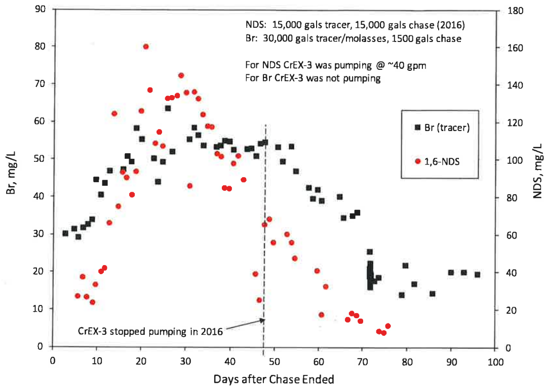
Figure 14 Comparison of responses of bromide in 2017 molasses test and 1,6-NDS in 2016 tracer test in R-28. Both tracers were passively sampled after injection into R-28. Details of the injections are provided at the top of the plot. Well CrEX-3 was not pumped during the 2017 molasses test.
