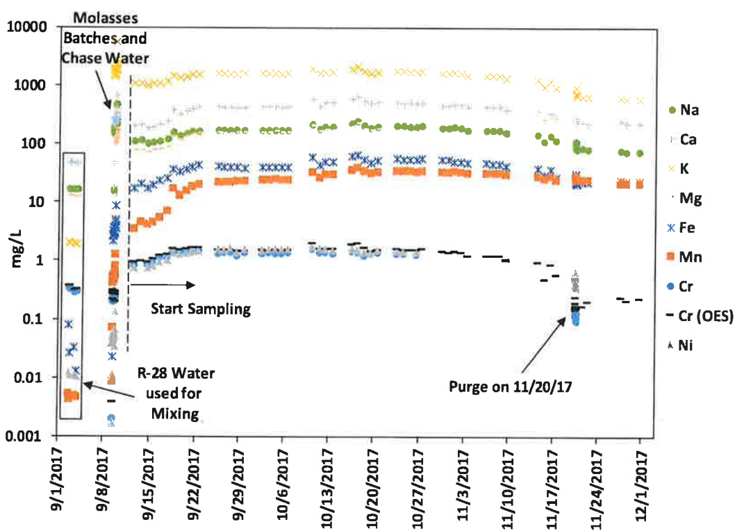
Figure 9 Concentrations of selected cations and metals in R-28 molasses test as a function of time. The more reliable analytical results for chromium (ICP-MS) are lagging, so chromium results from ICP-OES are also shown.
