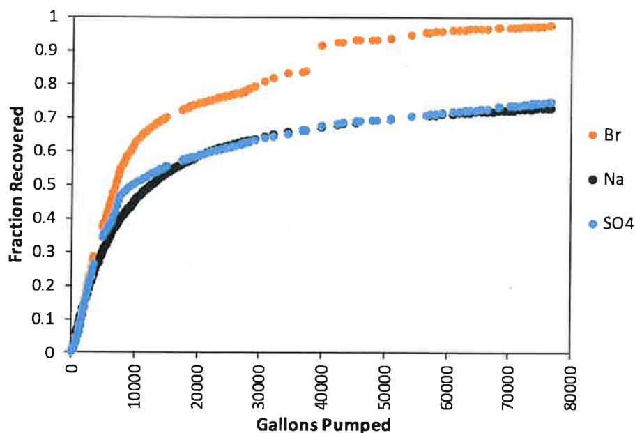
Figure 7 Fractional recoveries of bromide, sodium, and sulfate as a function of volume pumped from R-42. Sulfate recovery is based on assuming 2 M of sulfate generated for every mole of dithionite injected, and 1 M of sulfate for every mole of sulfite injected.
