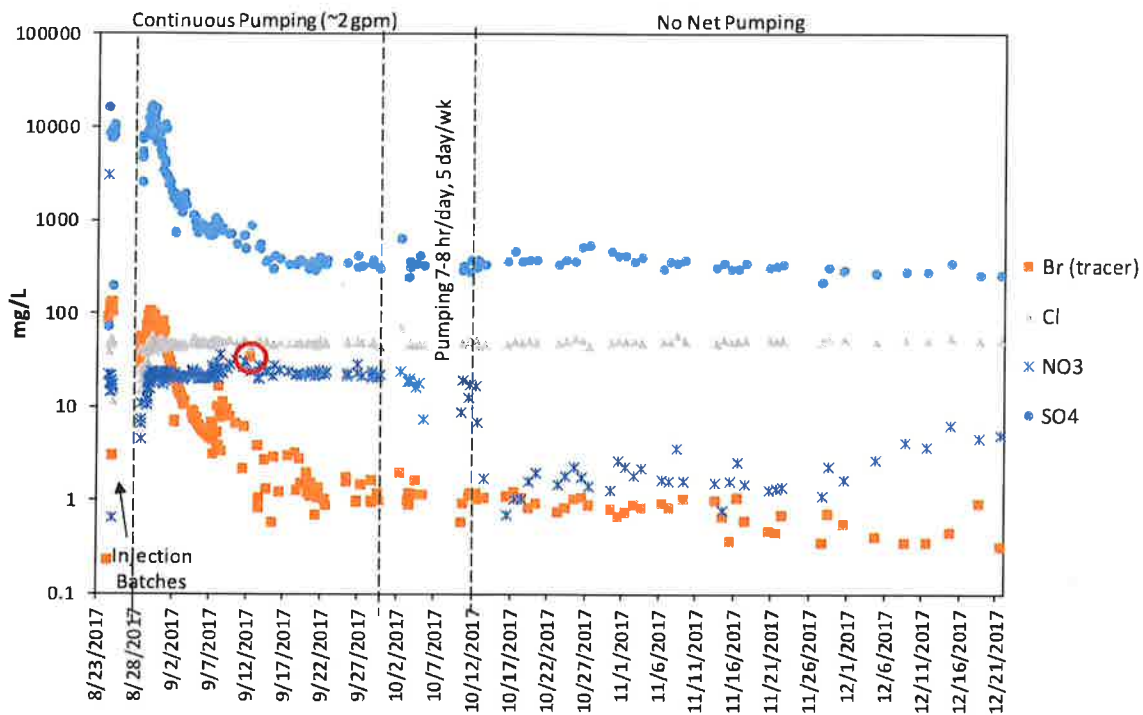
Figure 5 Concentrations of anions in R-42 dithionite test as a function of time. Circled bromide point causes a significant discontinuity in bromide recovery curve (Figure 7), but it was verified by two repeat analyses.
