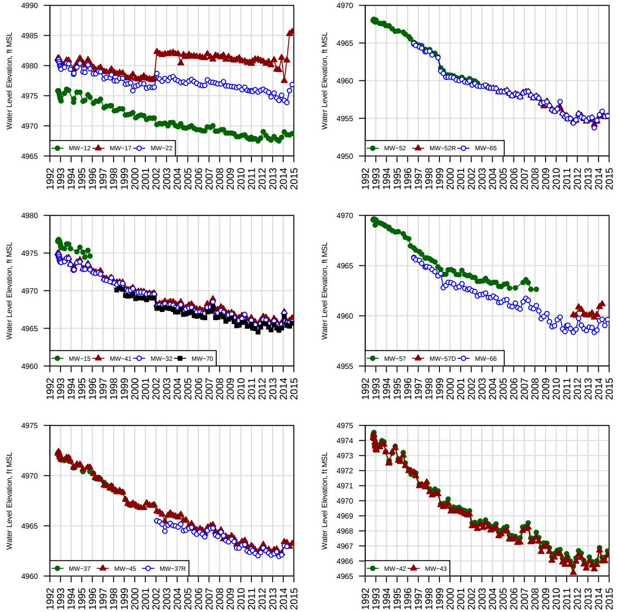
Figure 3.1: Monitoring Well Hydrographs
