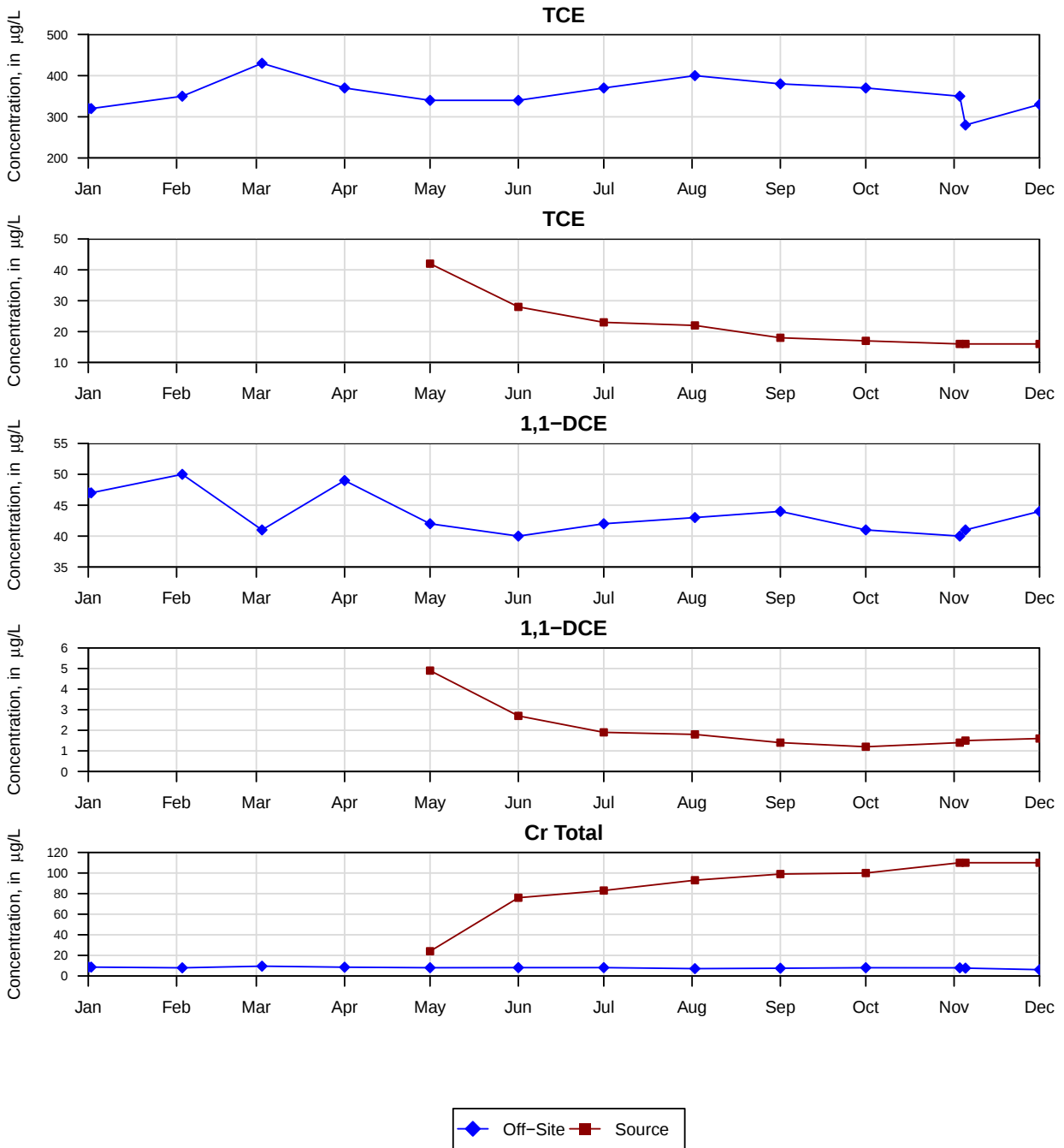
Figure 4.22: Off-Site and Source Containment Systems - TCE, DCE, and Total Chromium Concentrations in the Influent - 2014
