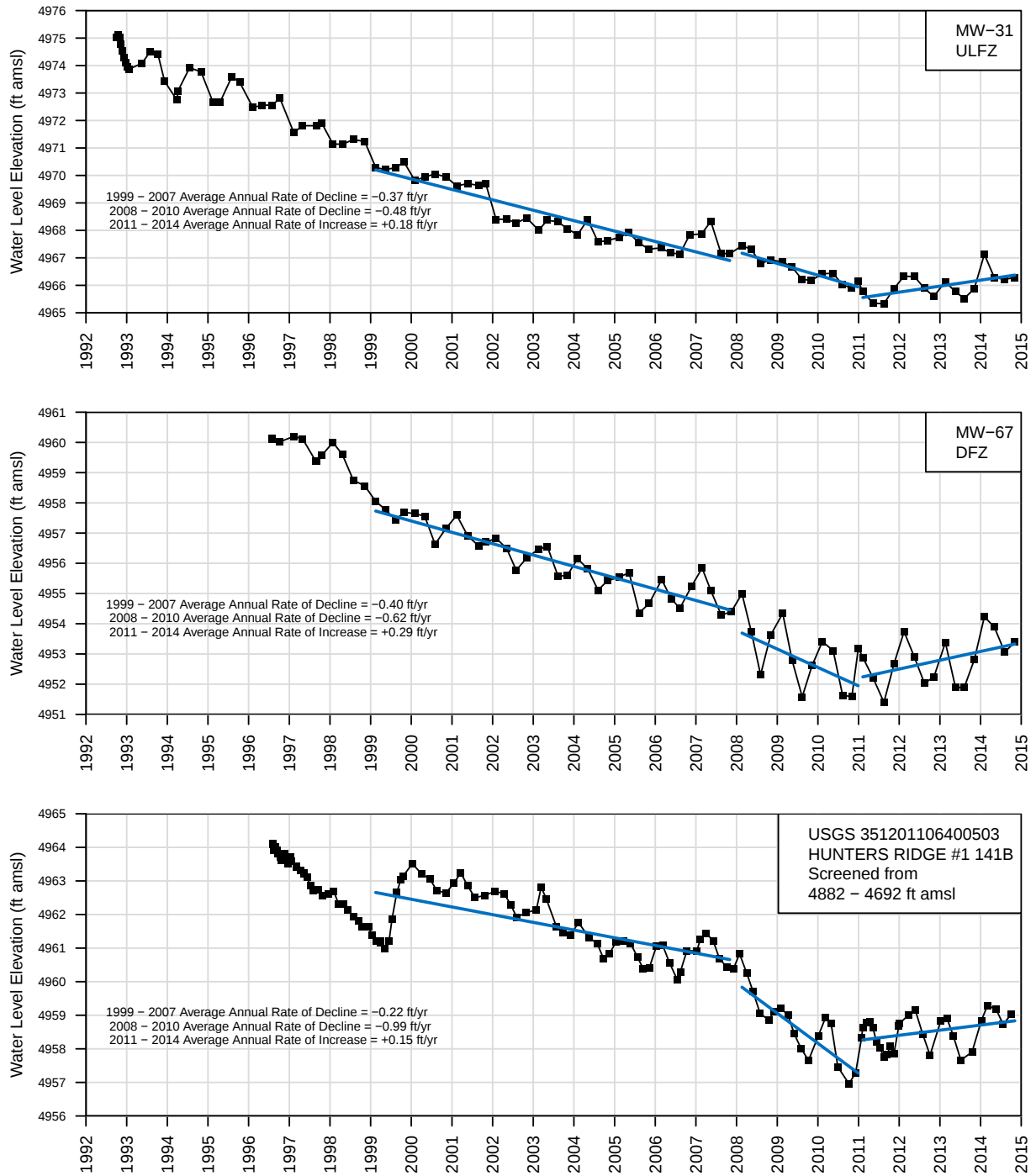
Figure 5.3: Regional Water-Level Trends
