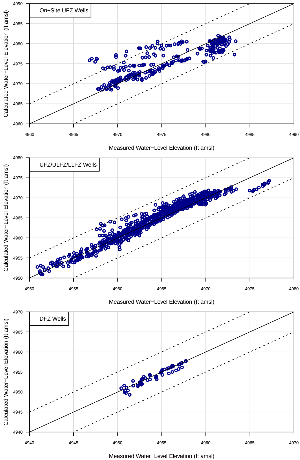
Figure 5.7: Comparison of Calculated to Observed Water-Levels - November 1998 through November 2014
