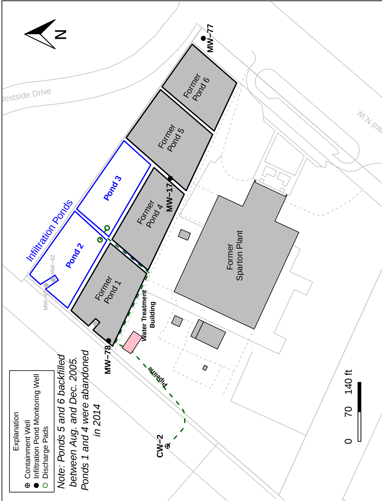
Figure 1.8: Layout of the Source Containment System
