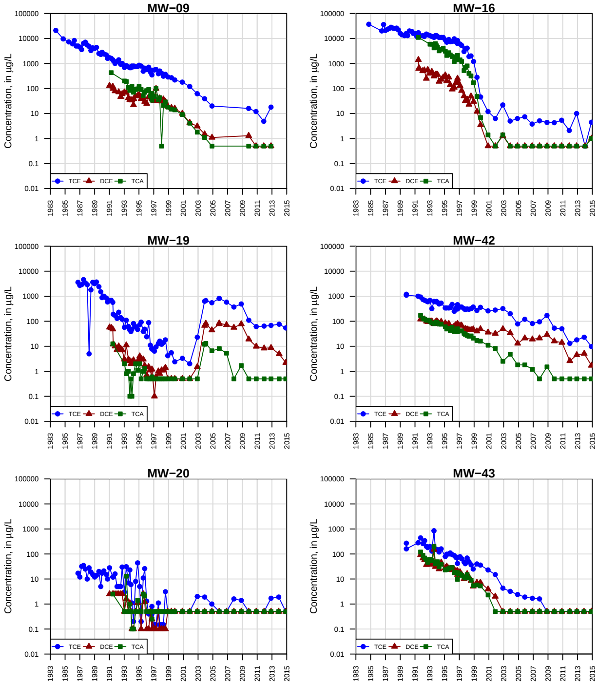
Figure 4.14: Contaminant Concentration Trends in On-Site Monitoring Wells
