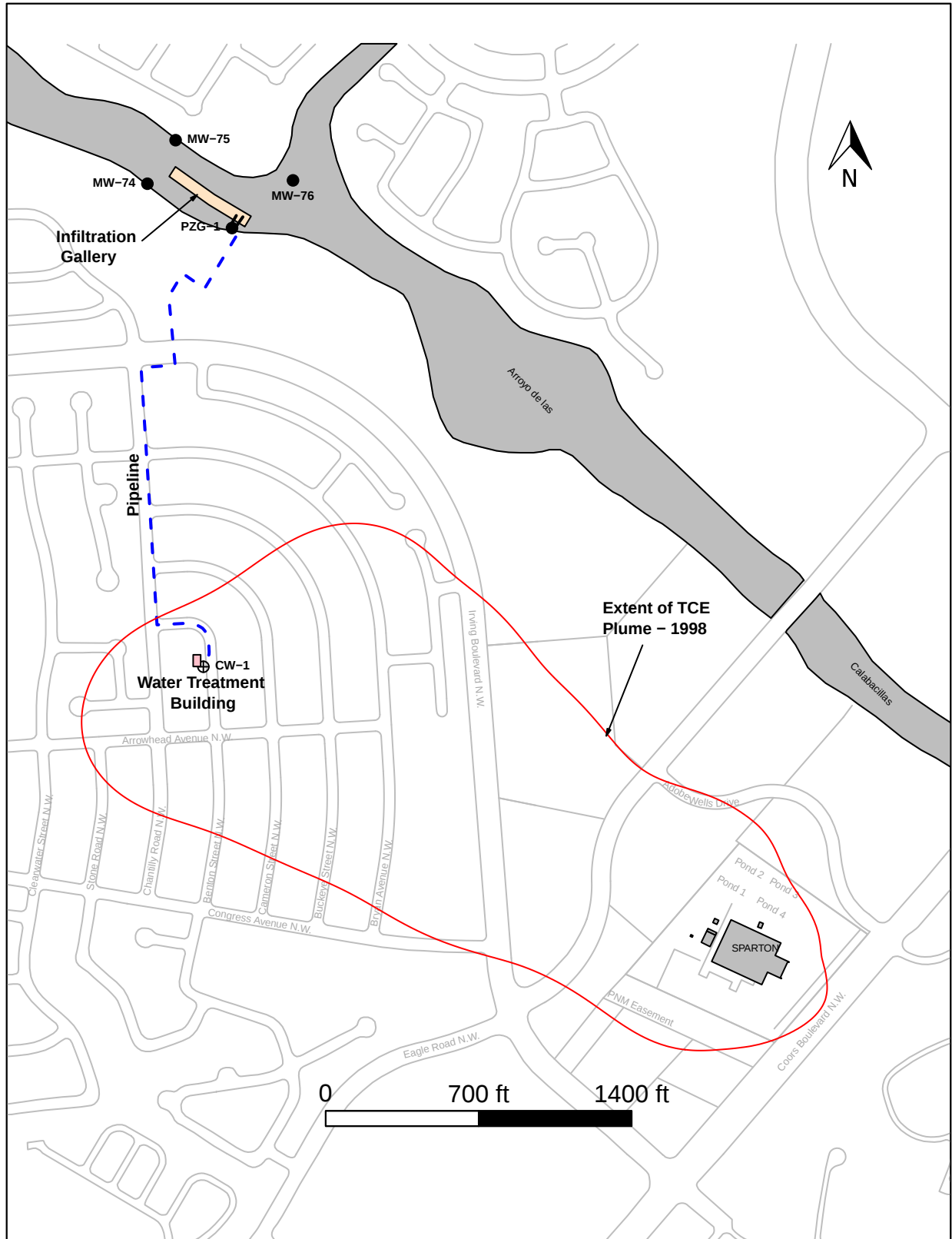
Figure 1.7: Layout of the Off-Site Containment System
