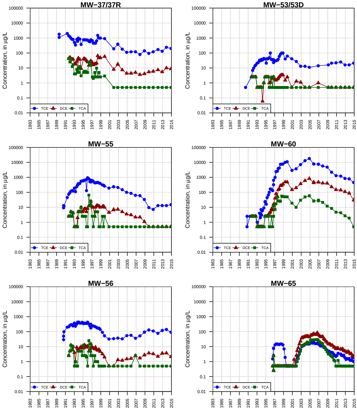
Figure 4.15: Contaminant Concentration Trends in Off-Site Monitoring Wells
