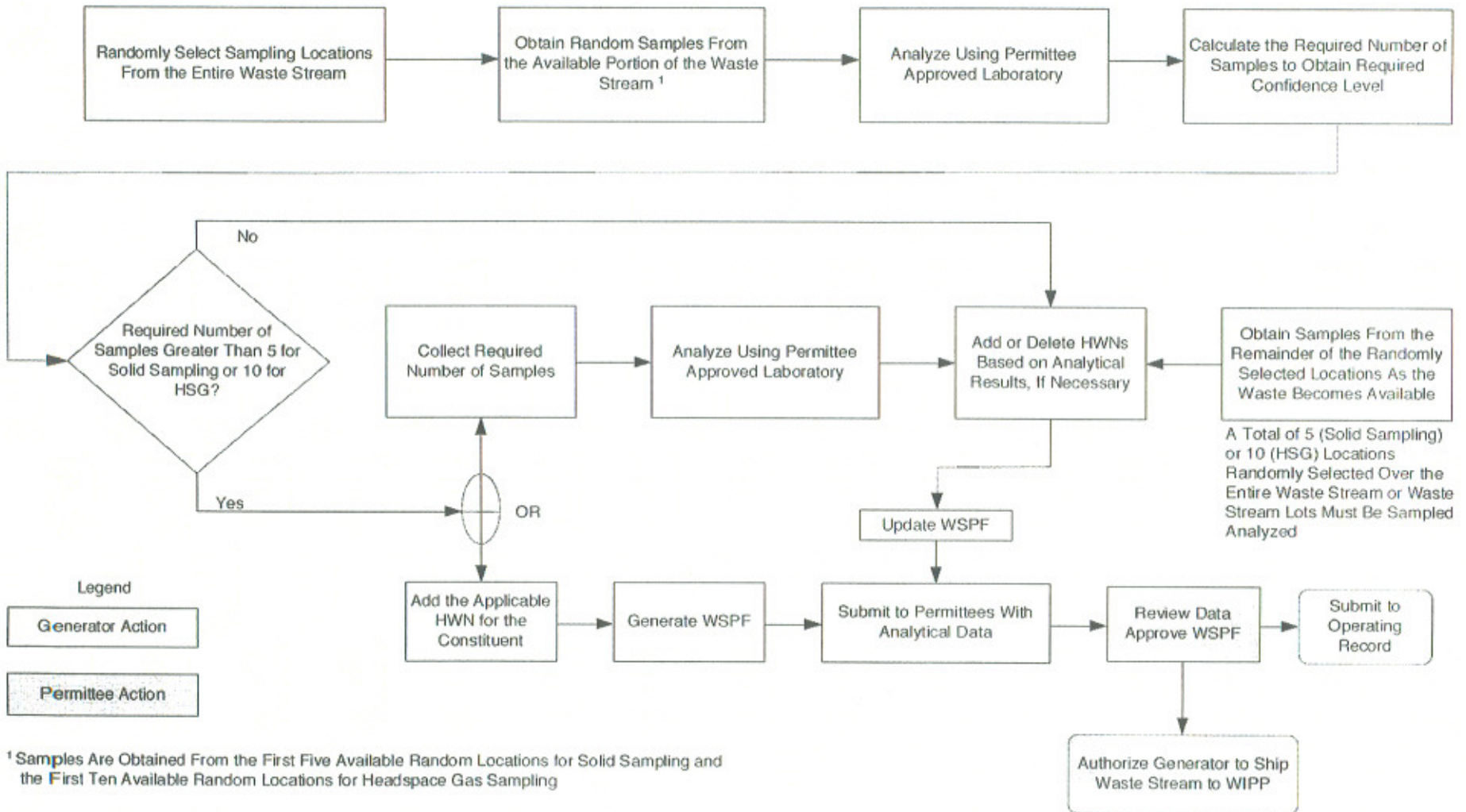
Figure B2-1 Statistical Approach to for Solid and Headspace Gas Sampling and Analysis of Waste Streams of Retrievably Stored Homogeneous Solids and Solid/Gravel to Obtain Additional Waste Characterization Information
