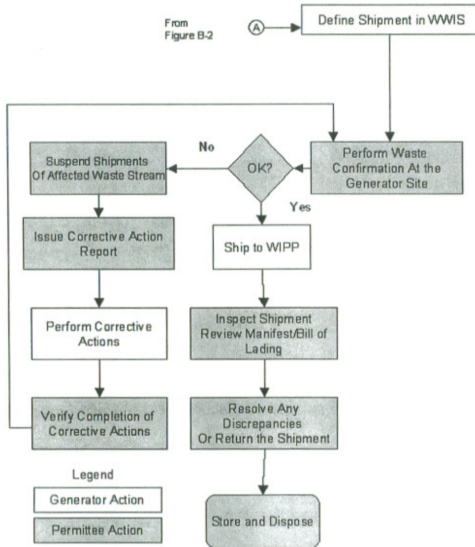
Figure B7-1 Waste Confirmation Process
