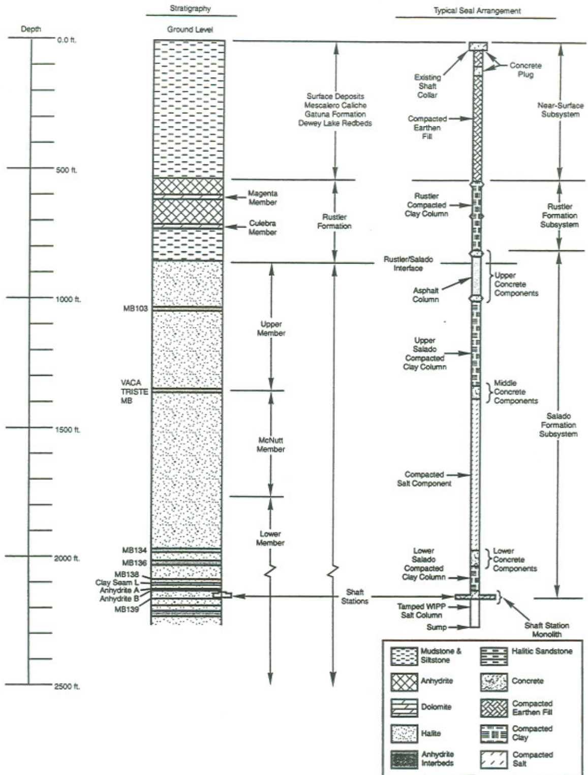
Figure J1-3 Typical Shaft Sealing System
