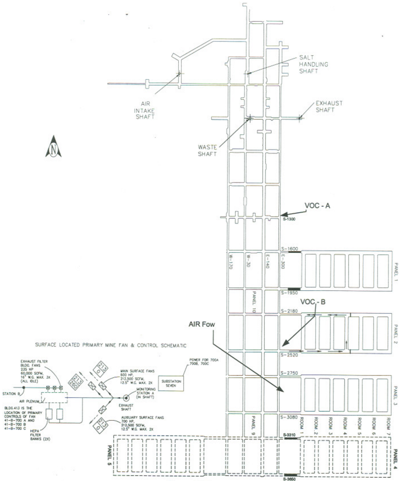
Figure N-1 Panel Area Flow
