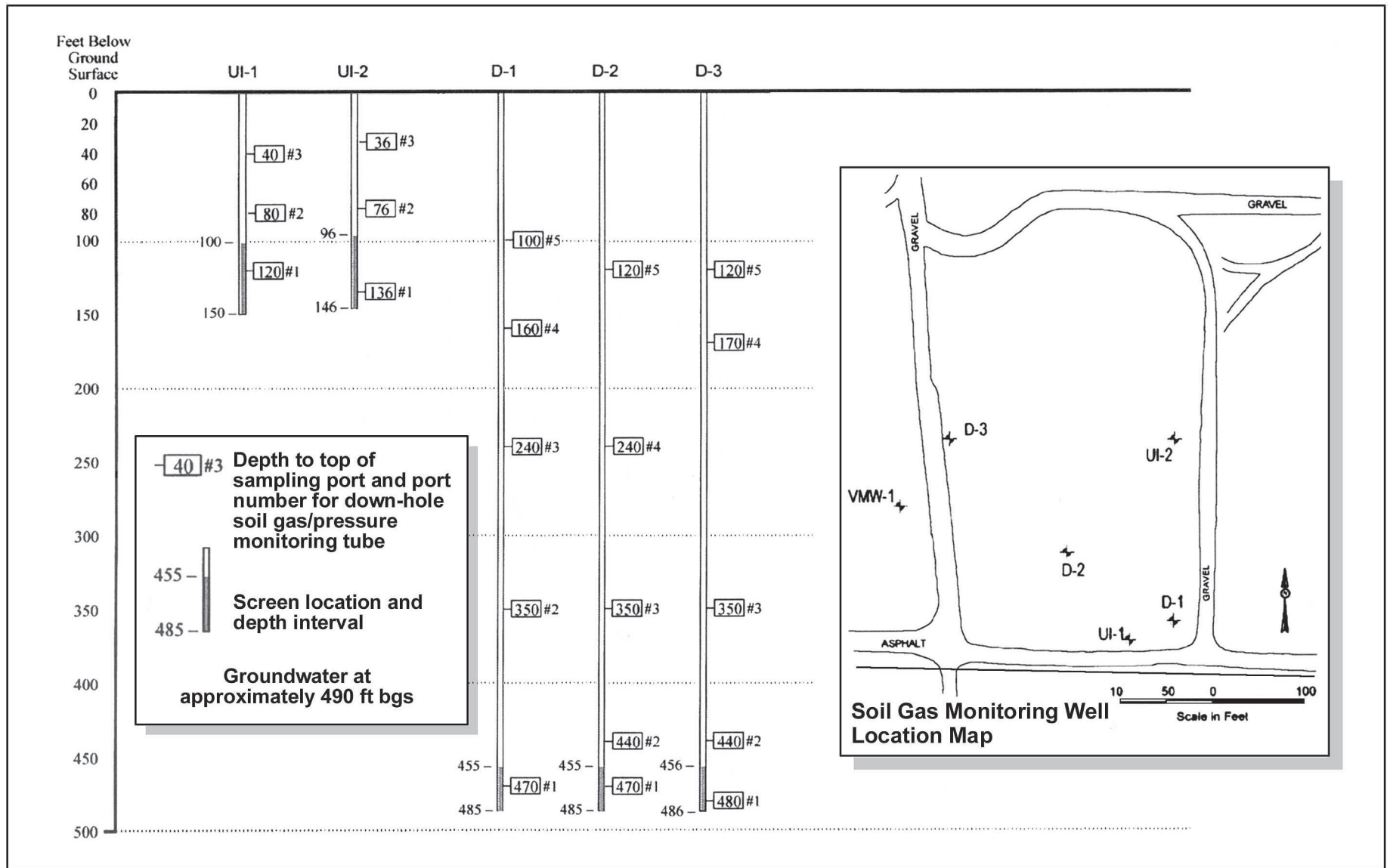
Figure 10 Soil-Gas Monitoring Wells and Depth-Specific Sampling Ports Chemical Waste Landfill
