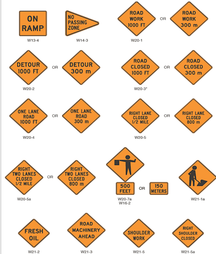
Figure 6F-4. Warning Signs in Temporary Traffic Control Zones (Sheet 3 of 4)
