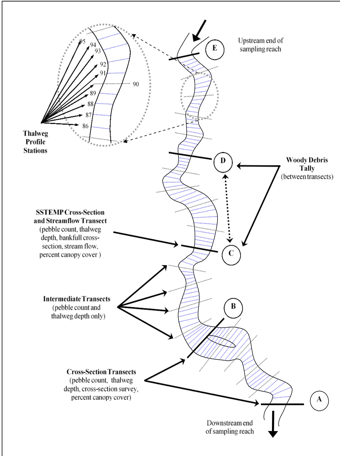
Figure 1. Reach layout for physical habitat measurements, record location of Transect A and E w/GPS
