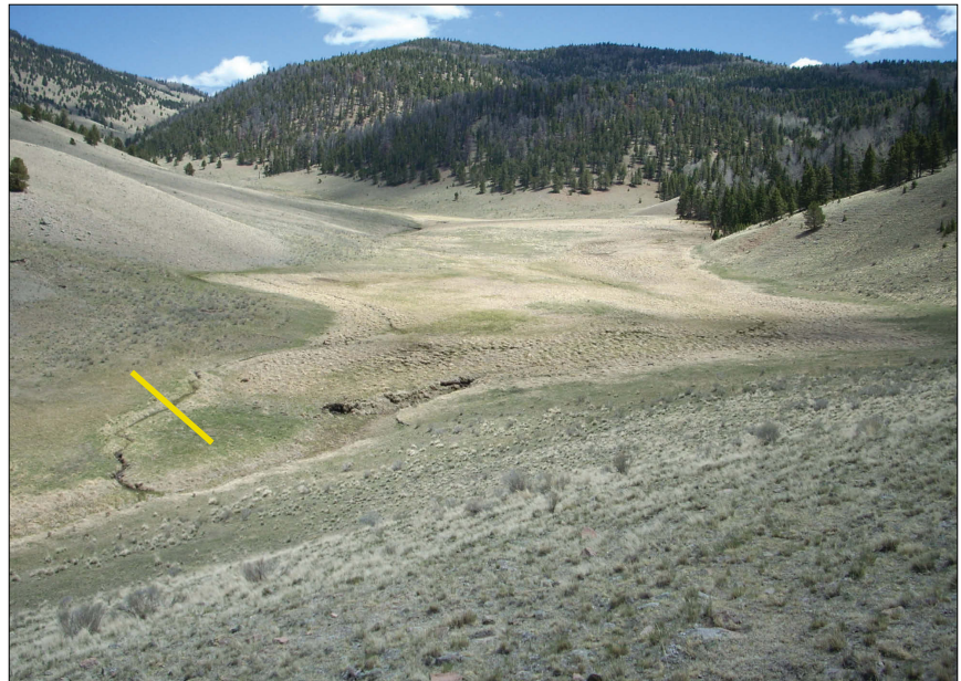
Figure 25. Headwater slope wetland complex in No Name Creek drainage, Carson National Forest, showing slope wetland progression and erosion. The yellow line shows a transect where soil samples were collected.
