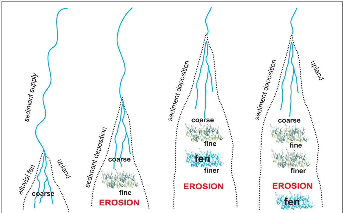
Figure 28. In this schematic of slope wetland progression, aggrading sediment causes formation of the headwater slope wetland complex. The downslope toe is continually eroding. The presence of a fen is dependent upon site hydrology and fens are not present in all headwater slope wetland complexes.
