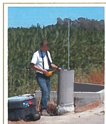
A hand held meter mounted on a rod works well for measuring flow velocity at a single point in time. The velocity should be measured at several points across the transect of the pipe if using an electromagnetic or propeller meter.
