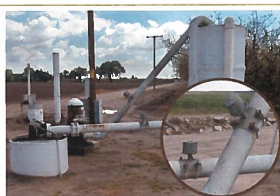
Inexpensive propeller meters are well suited for measuring pumped groundwater or clean district water but can easily foul if debris is present.
