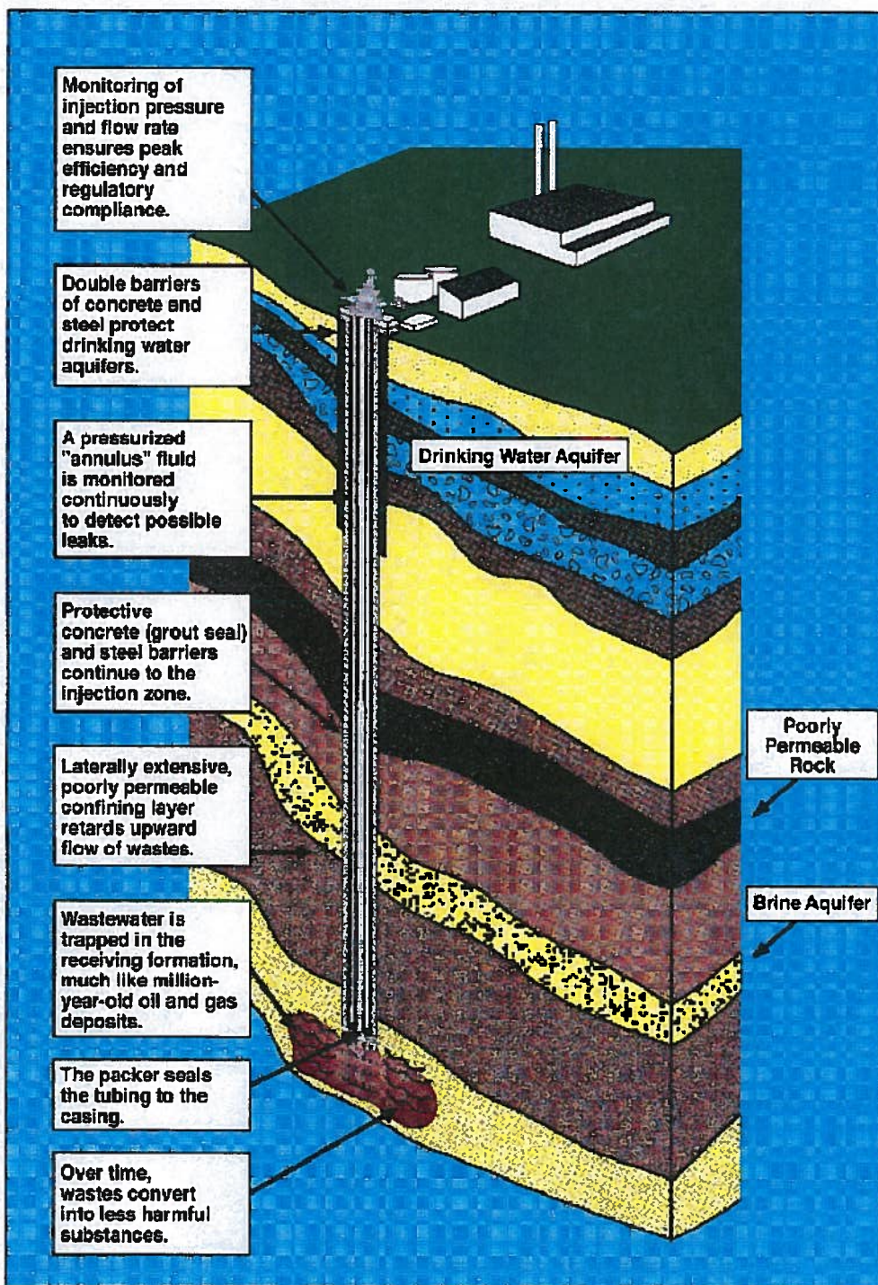
Exhibit 3 A Typical Class I Injection Well
