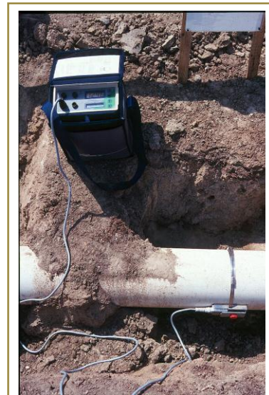
Clamp on Doppler meters do not require cutting into the pipe making them ideal for temporary installations. Their stringent placement requirements limit their use on dairies.
