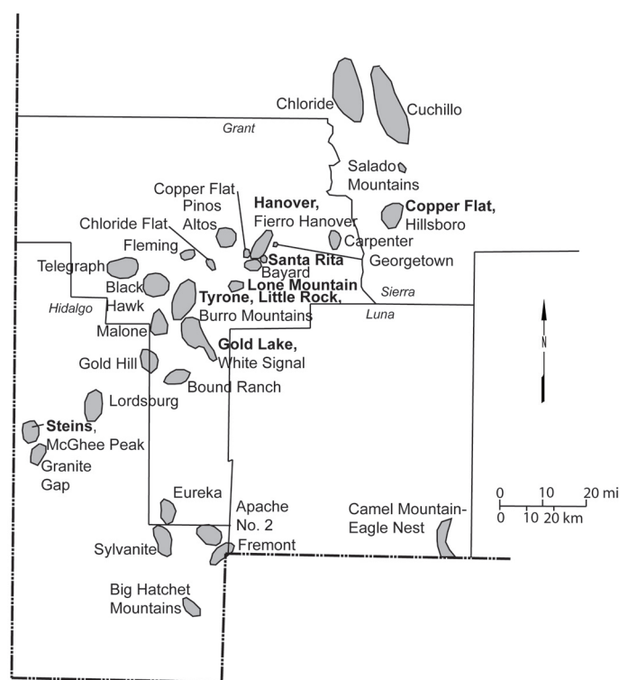
FIGURE 2. Laramide mineral deposits and plutons in southwestern New Mexico.
