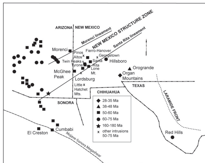
FIGURE 1. Laramide porphyry copper deposits in southwestern United States and northern Mexico.
