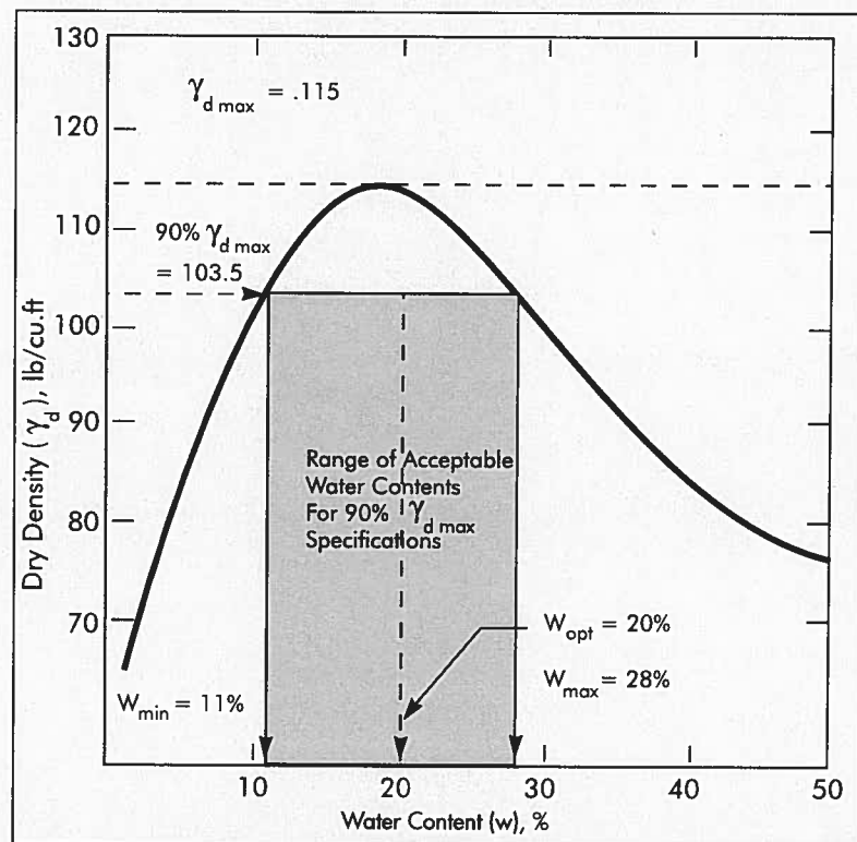
Water Content for Achieving a Specific Density
