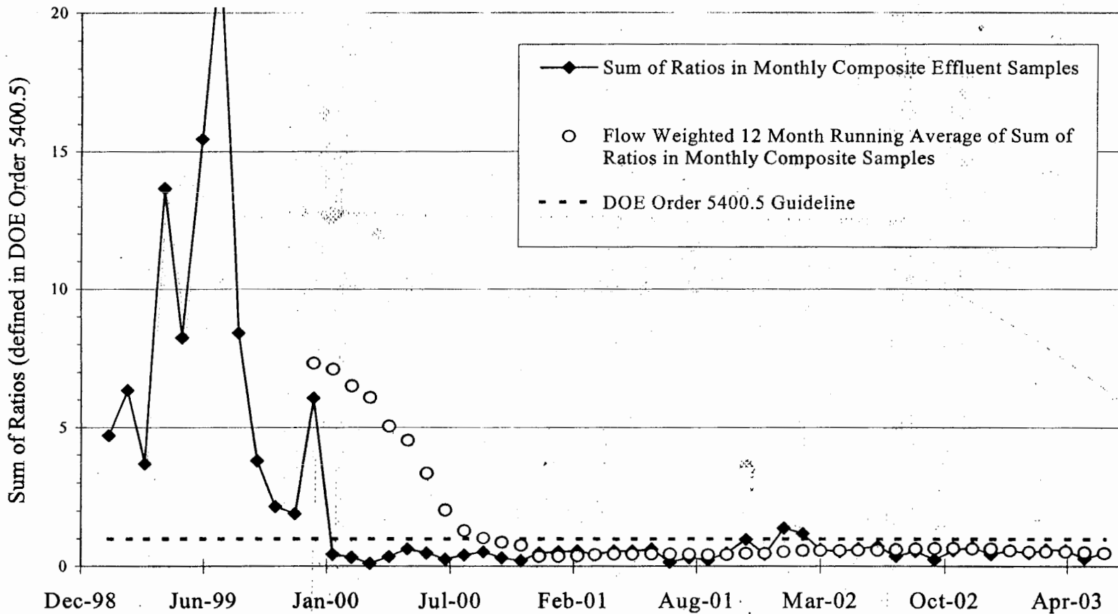
Monthly and 12 Month Running Average of RLWTF Effluent from December 1998 through June 2003 (55 months) Analysis of Flow Weighted Monthly Composite Samples
