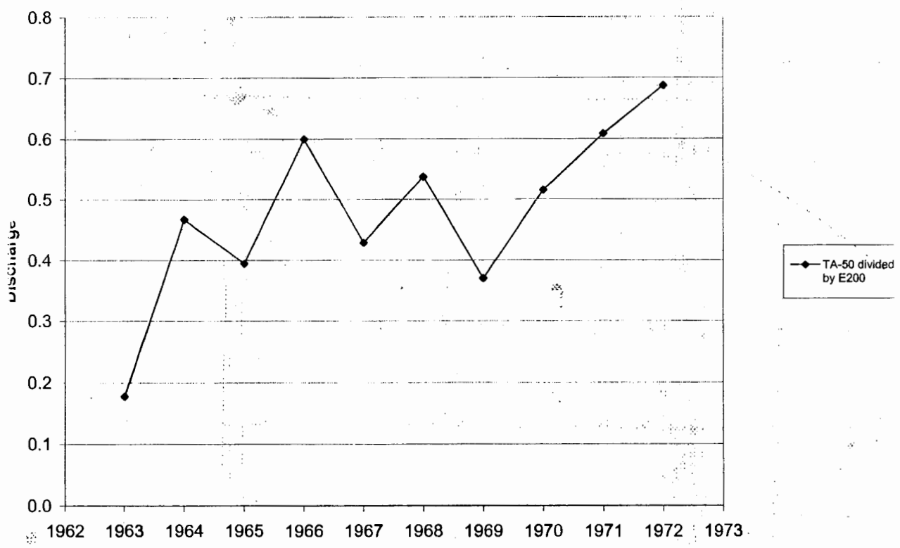
TA-50 Portion of Annual Discharge Volumes Mortandad Canyon 1963-1972 Average Ratio: 0.51
