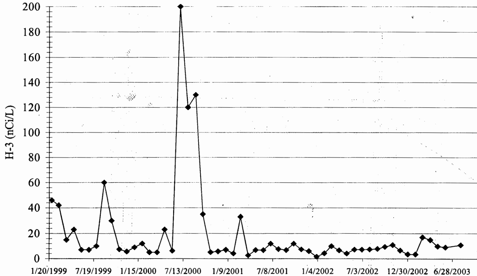
Tritium in Final Monthly Composite Samples (1/99 - 7/03)
