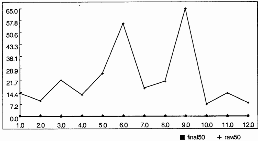
RAW50 and FINAL50 Pu-239 concentration (nCi/L). JAN-2002 through DEC-2002
