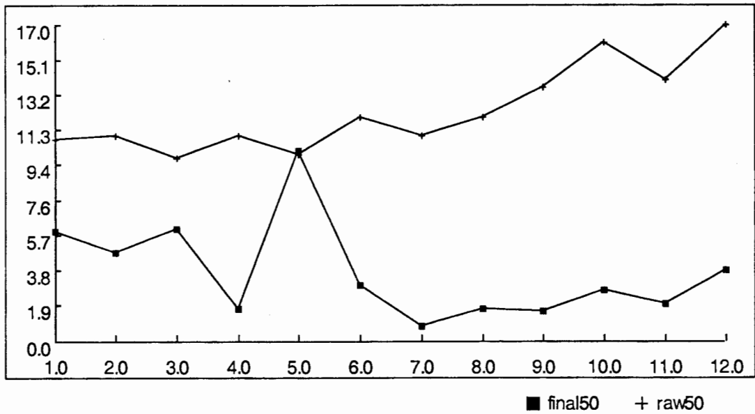
RAW50 and FINAL50 CALCIUM concentration (mg/L). JAN-2002 through DEC-2002
