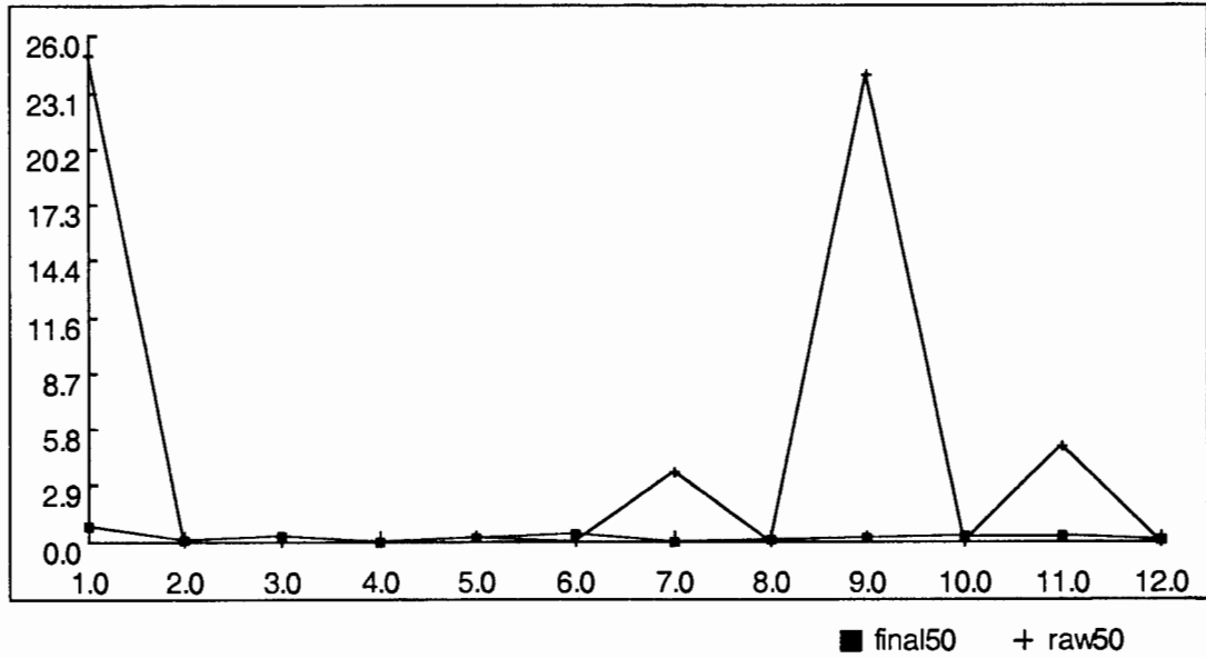
RAW50 and FINAL50 BETA concentration (nCi/L). JAN-2002 through DEC-2002
