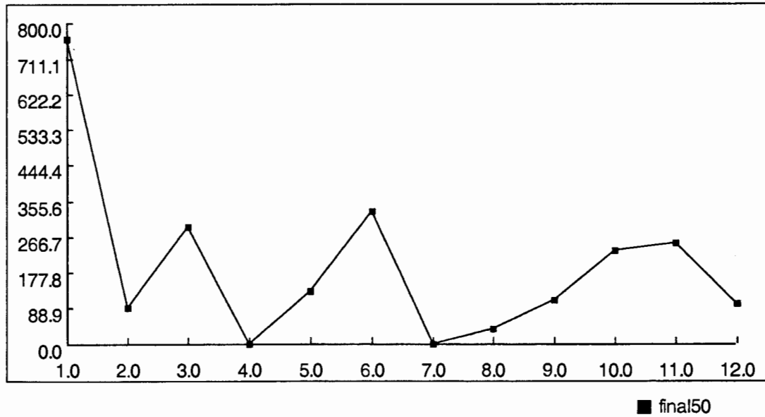
FINAL50 BETA concentration (pCi/L). JAN-2002 through DEC-2002
