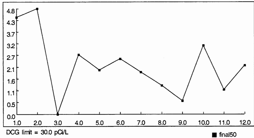
FINAL50 Pu-239 concentration (pCi/L). JAN-2002 through DEC-2002
