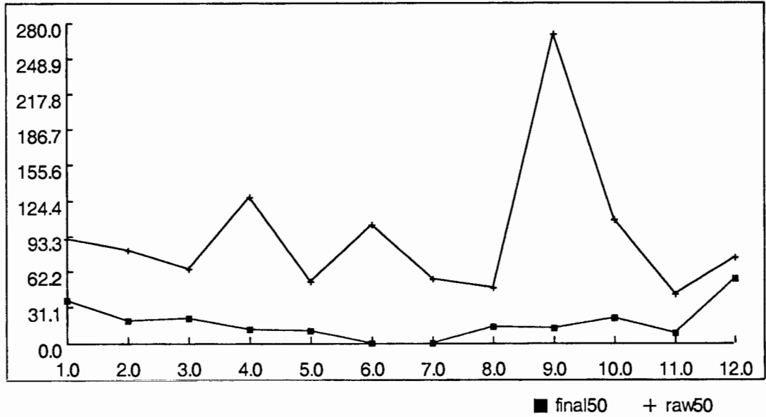
RAW50 and FINAL50 COD concentration (mg/L). JAN-2002 through DEC-2002
