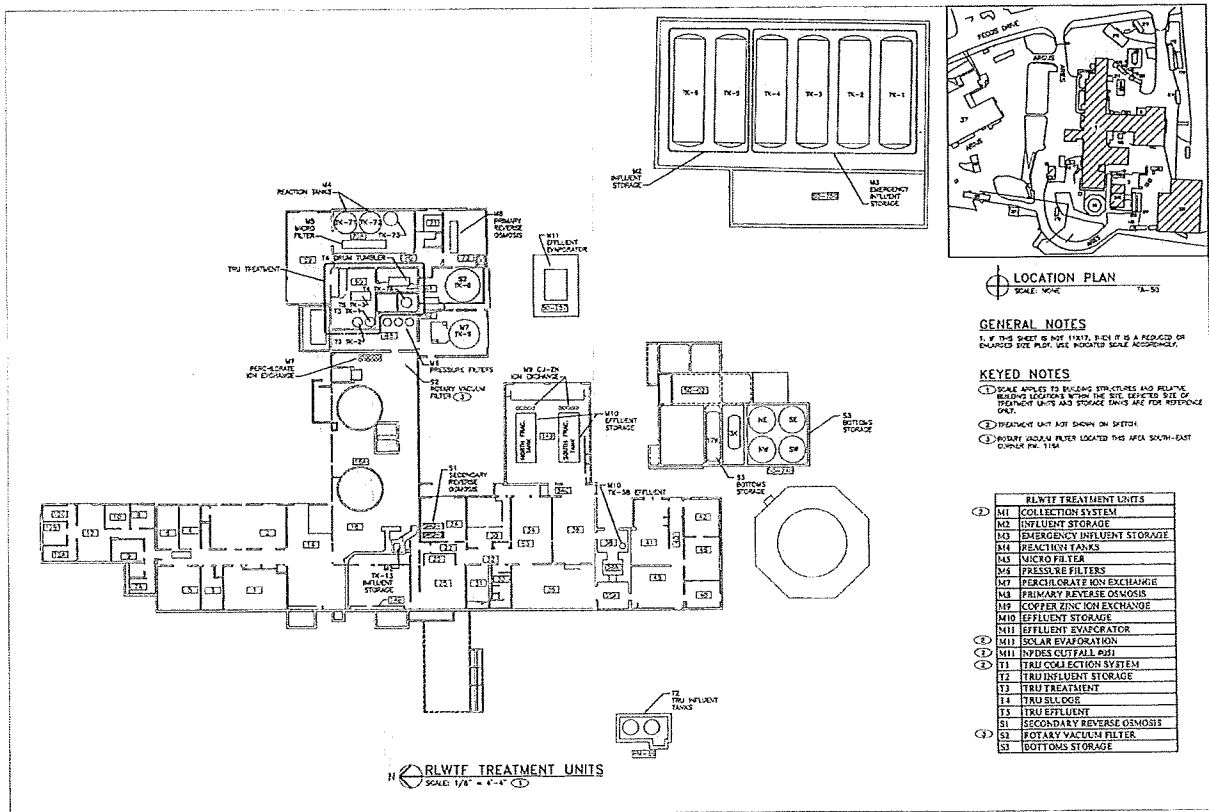
Figure 2. RLWTF Location and Treatment Units
