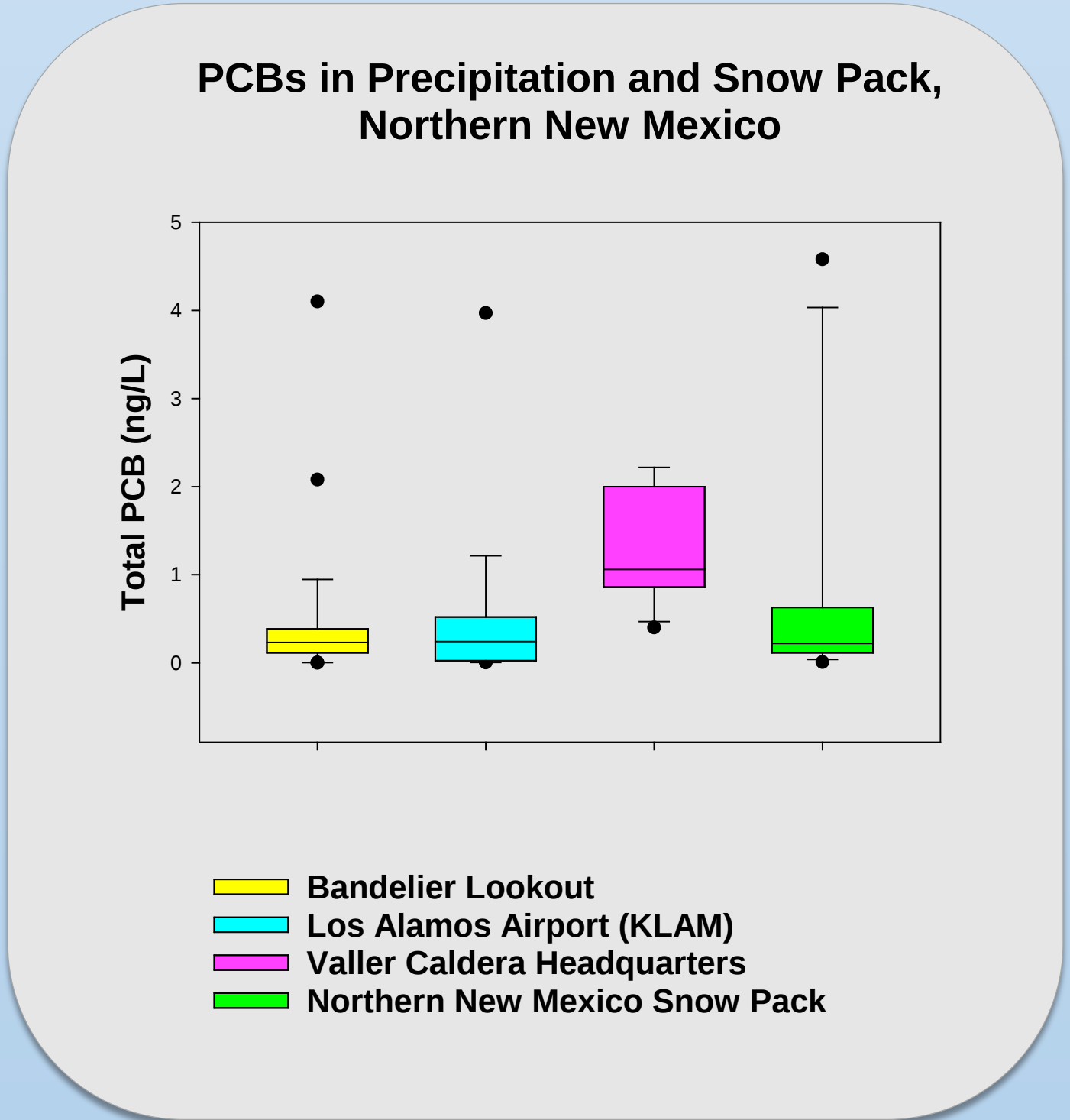
Figure 4. Box plots of PCB results in precipitation and snowpack.
