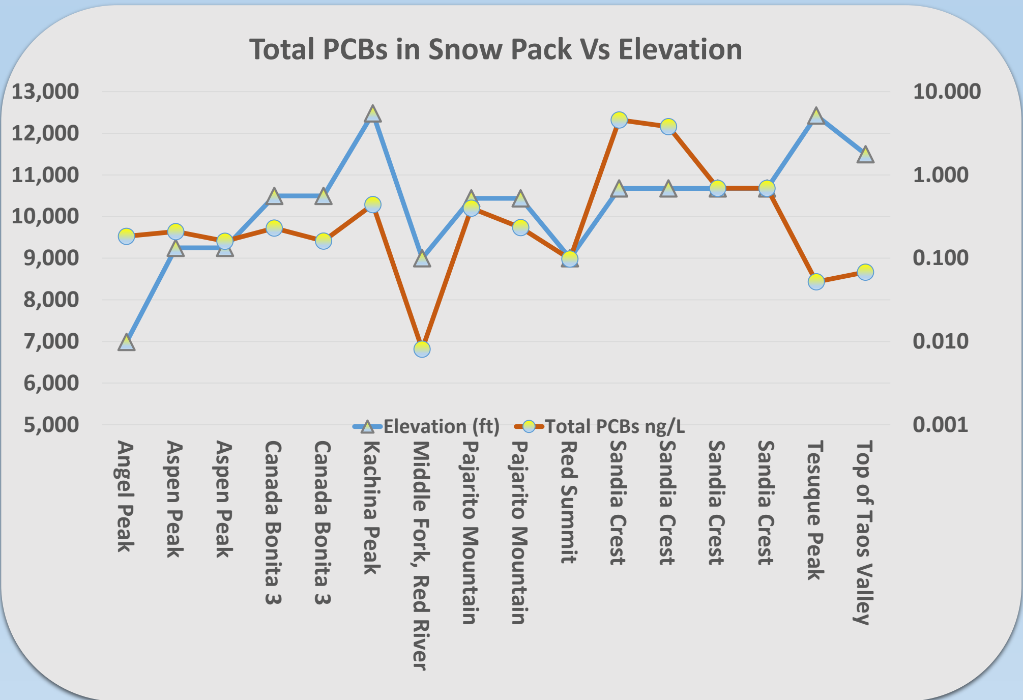
Figure 5. Plot of altitude and PCB concentrations in snowpack, northern New Mexico.
