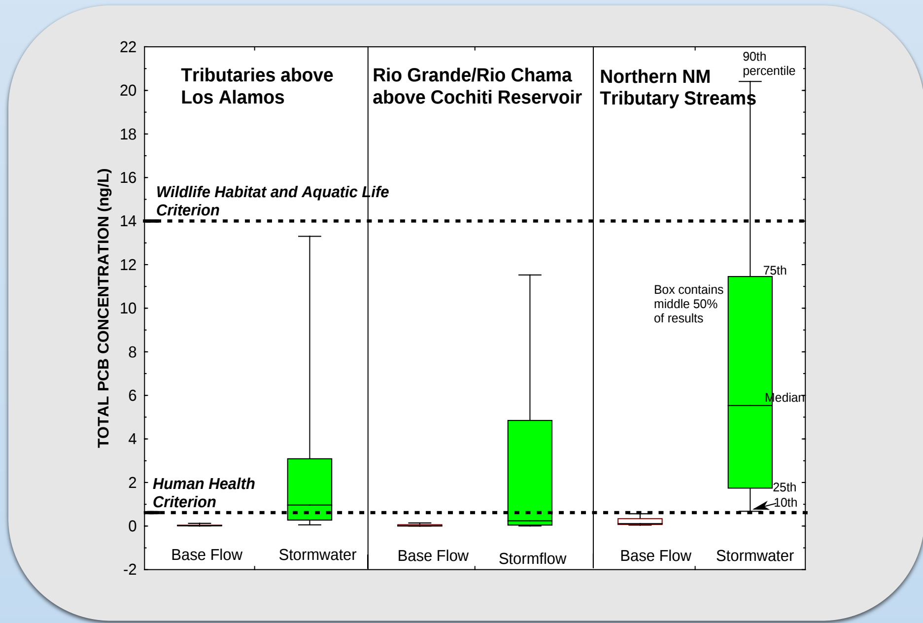
Figure 1. Box plots of base flow and storm water runoff PCB concentrations for various drainages in the upper Rio Grand system.
