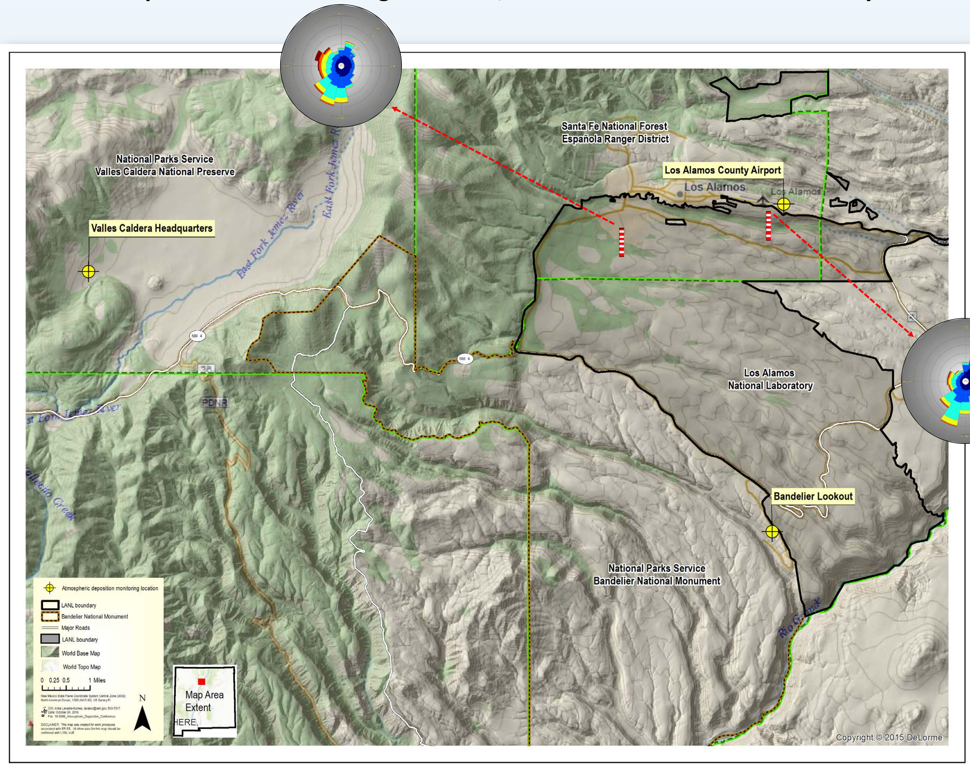
Figure 2. Map of the study area showing wind roses and monitoring locations.
