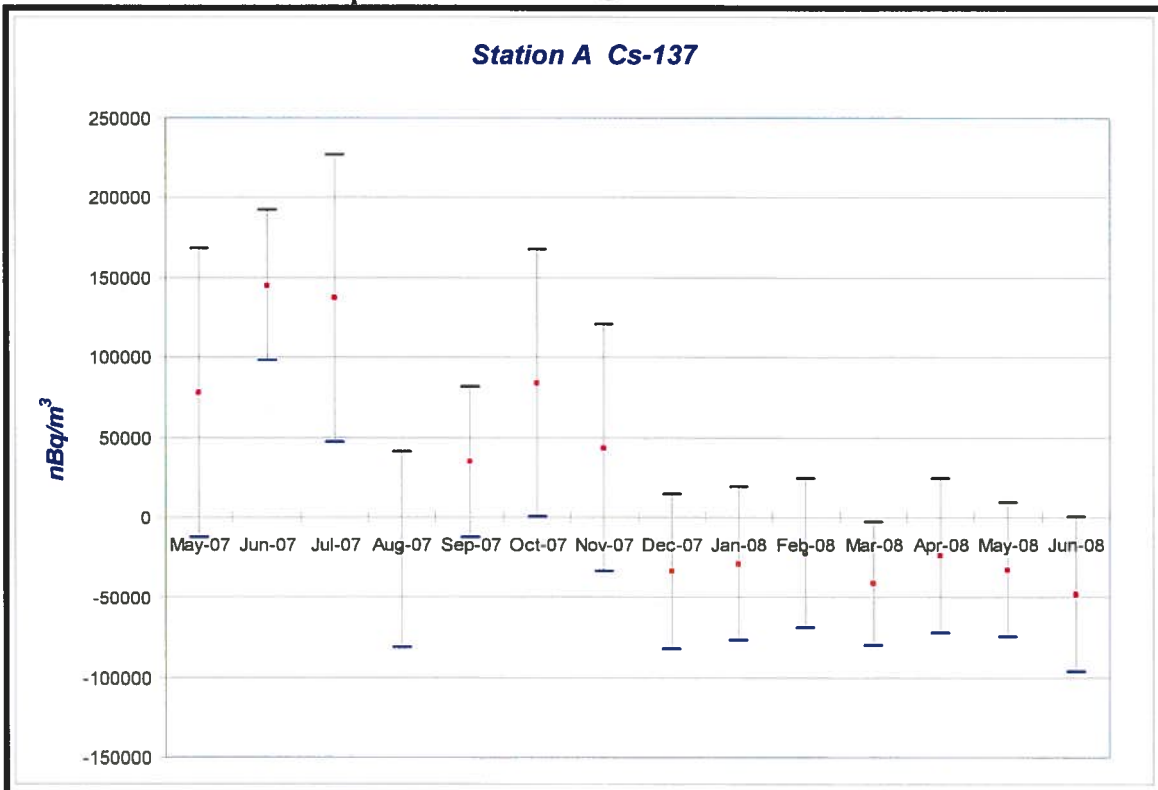
Graph 2: Lab Results for Cs-137 from Station A
