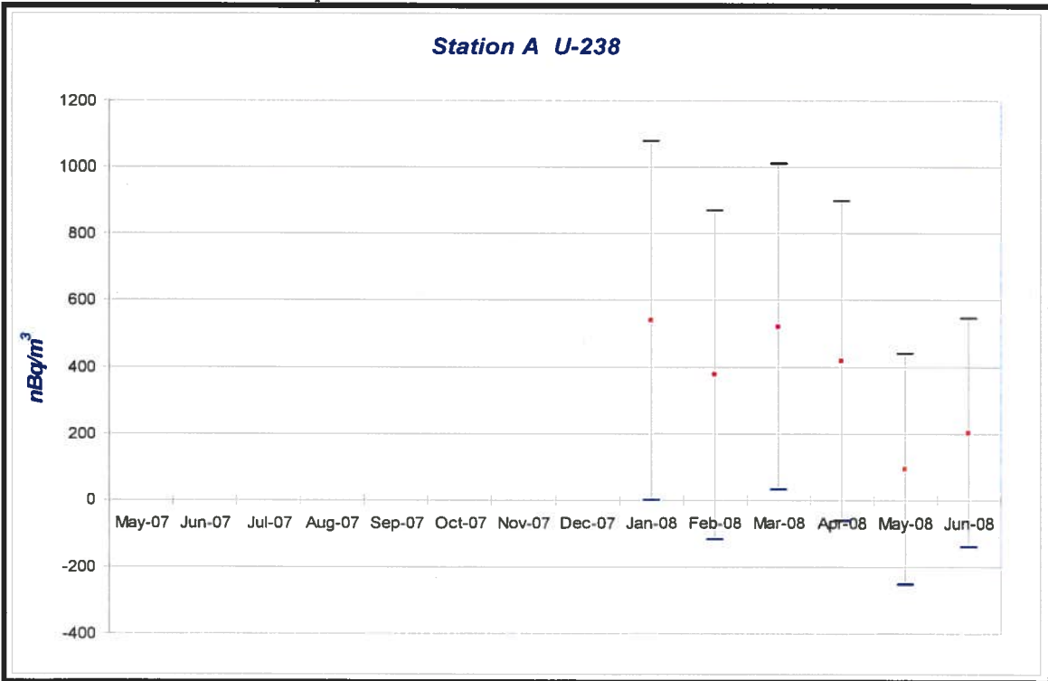
Graph 10: Lab Results for U-238 from Station A
