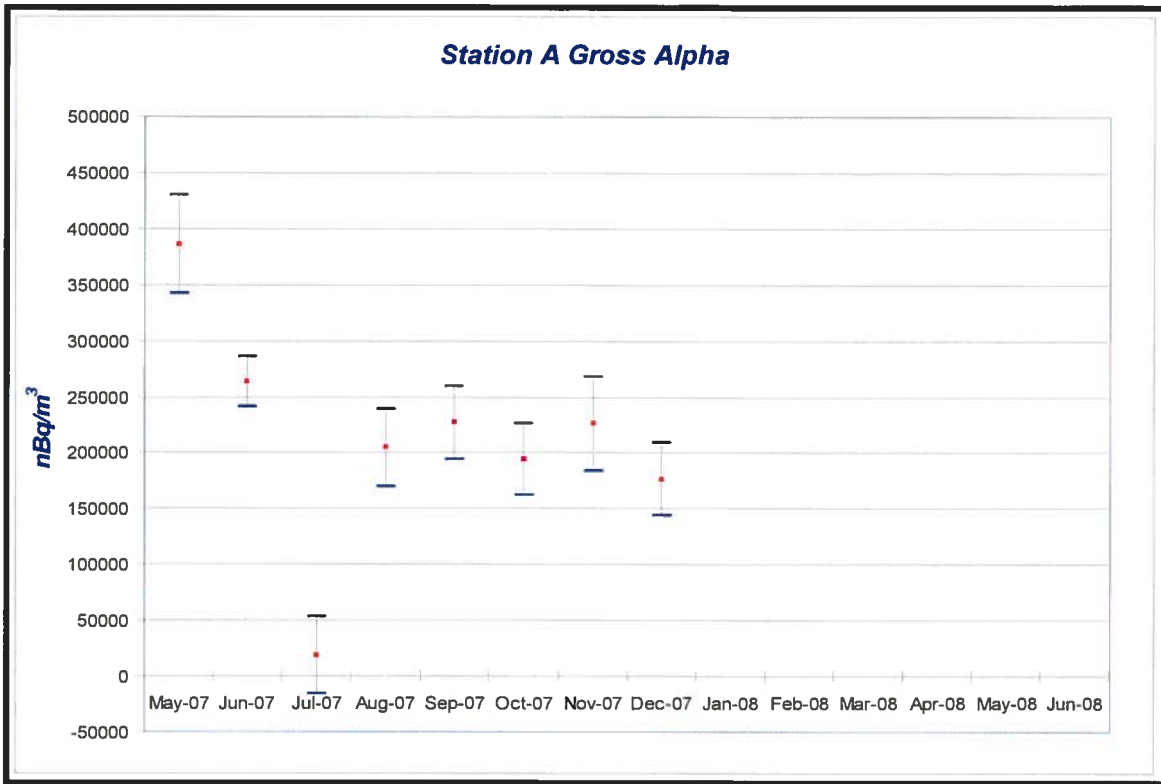
Graph 3: Lab Results for Gross Alpha from Station A
