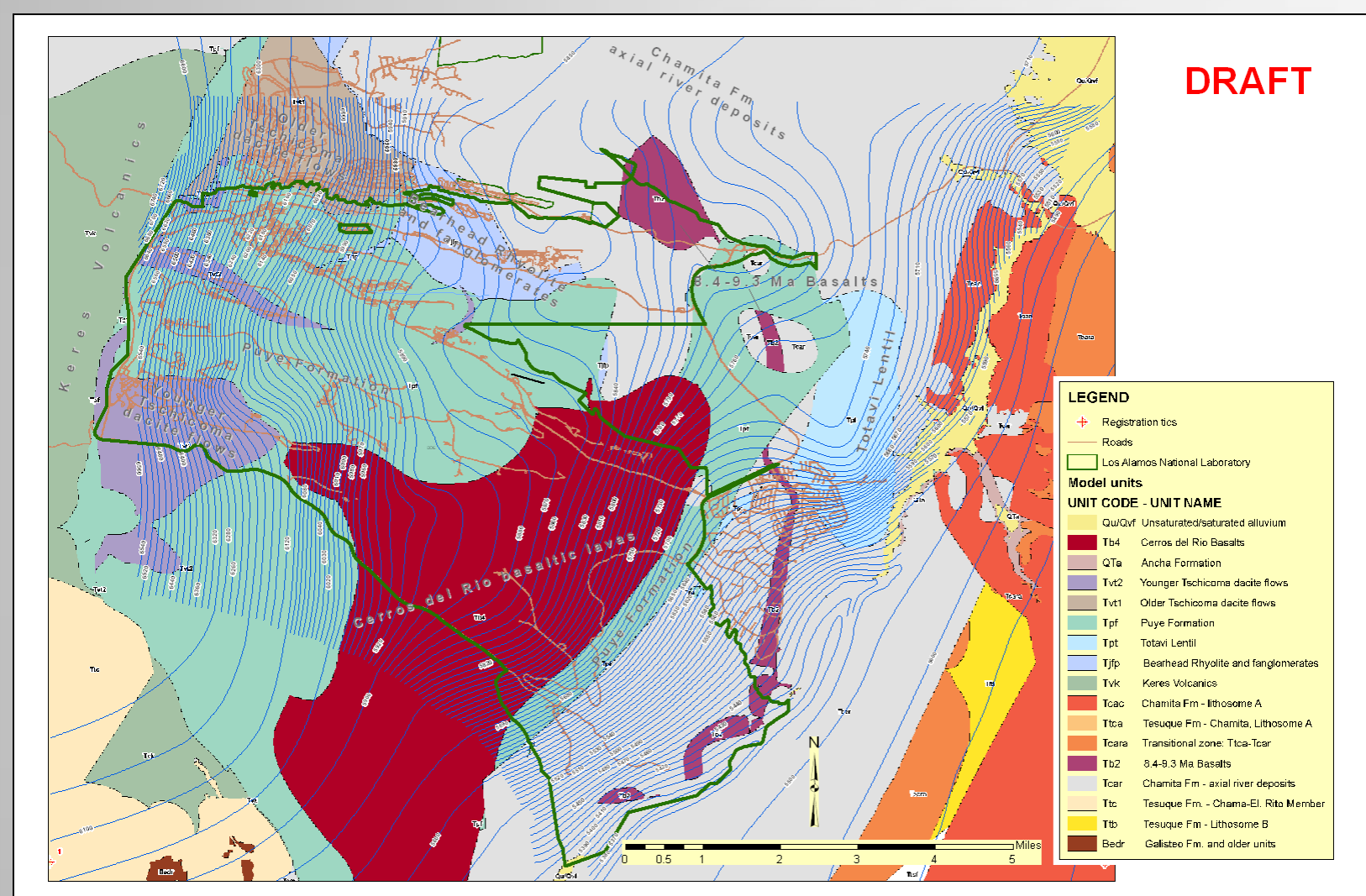
Geology at the water table and water-table elevation contours
