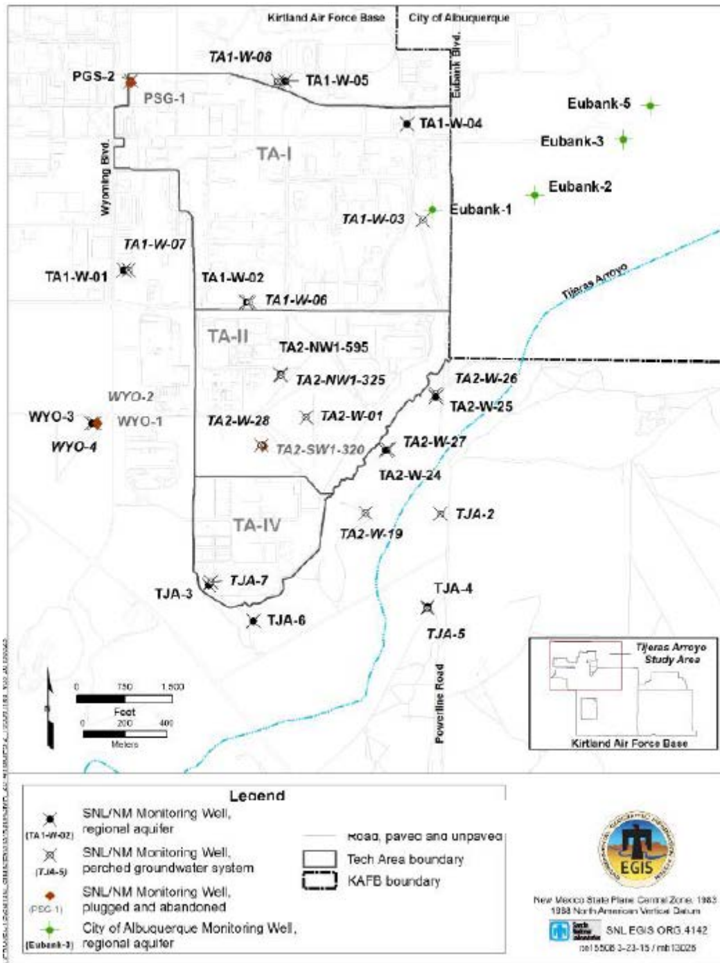
Figure 1. TAG Monitoring Well Locations (Sandia National Laboratories, New Mexico Environmental Geographic Information System, Annual Groundwater Monitoring Report, Calendar Year 2012)
